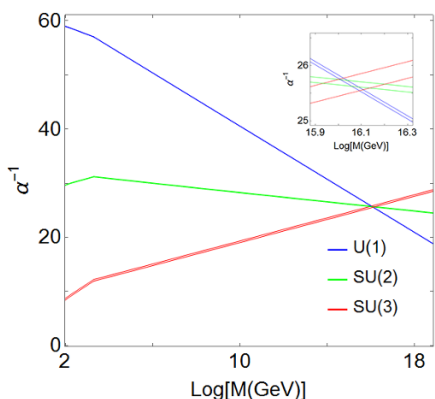
Figure 1. Running of the gauge couplings \alpha_1^{-1} (blue), \alpha_2^{-1} (green) and \alpha_3^{-1} (red) with M_{\text{SUSY}} = 2 \text{ TeV} up to 2-loop in \beta -functions. For each \alpha^{-1} it is reported the 3\sigma error band due to the experimental uncertainty at M_Z . The range for M_{\text{SUSY}} compatible with the measurements within 3\sigma is from \sim 1 \text{ TeV} up to \sim 3.5 \text{ TeV} . The inset is a focus of the crossing region.
