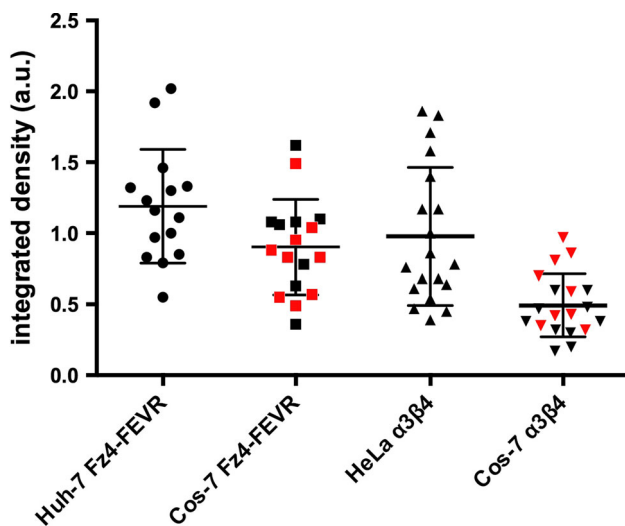
Fig. 4 Transfected Fz4-FEVR and \alpha 3\beta 4 are expressed in very similar amount in the different cell lines analyzed. Quantitation of the level of Fz4-FEVR or \alpha 3\beta 4 nAChR expressed in Huh-7 and COS-7 cells, and in HeLa and COS-7 cells, respectively. See “Materials and Methods” section for details. In red are indicated cells with perturbed ER. 47 % of the COS-7 cells expressing \alpha 3\beta 4 were not saturated. The Prism scattered dot blot is shown. The mean value and the standard deviation are indicated. Note that the average expression levels of Fz4-FEVR and \alpha 3\beta 4 are even higher in Huh-7 and HeLa cells, respectively, than in COS-7 cells (Color figure online)
