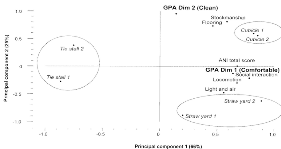
Principal Component Analysis: score and loading plot.
