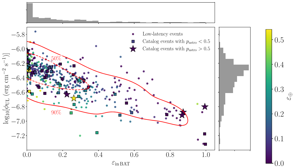
Figure 4. The 15–350 keV flux upper limit \phi_{\text{UL}} derived with NITRATES as a function of \varepsilon_{\text{in BAT}} , namely the probability that the GW candidate is contained inside the BAT FOV. The plot includes all the GW candidates received during O3, including both Burst and CBC events. With different symbols, we distinguish the GW candidates received in low latency and the ones confirmed and included in the O3 catalog, separated in p_{\text{astro}} > 0.5 and p_{\text{astro}} < 0.5 . The dashed and solid red lines are the 50% and 90% containment regions of the scatter plot, respectively. The one-dimensional histograms of \phi_{\text{UL}} and \varepsilon_{\text{in BAT}} are reported on the sides. The color bar indicates the value of \varepsilon_{\oplus} , the probability that the GW candidate is occulted by the Earth.
