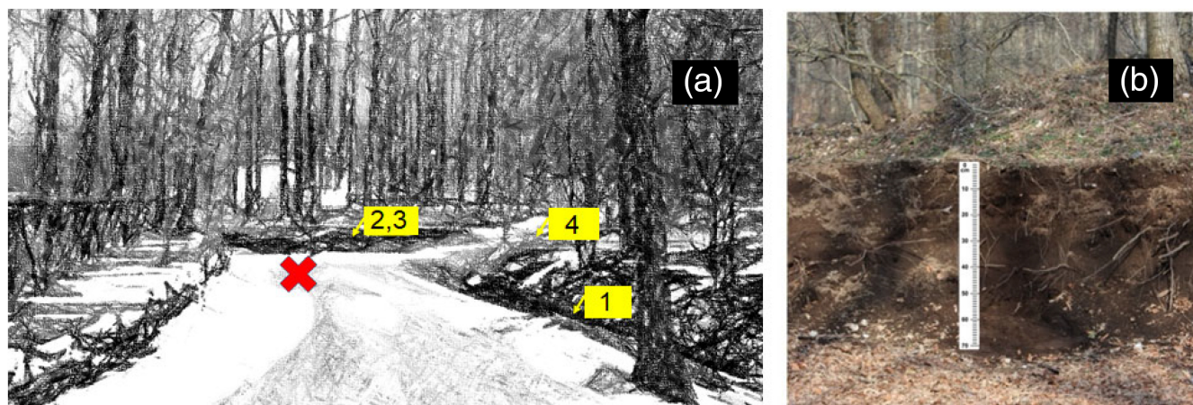
FIGURE 1 (a) Sketch of the crime scene setting (in white due to the snow cover, with a red cross marked as the location of where the body was found). The boxes in yellow denote the reference sampling locations. (b) A soil profile (from location 1) at the crime scene showing the dark A horizon.
