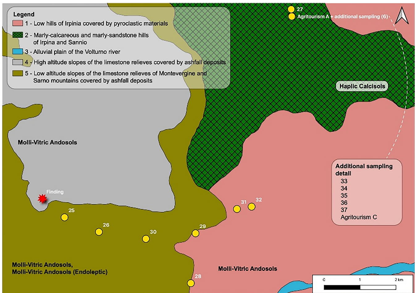
FIGURE 7 Map of land systems. Land system 2 (green with cross bars) is the main land system of interest Haplic Calcisols (IUSS Working Group WRB, 2022).
