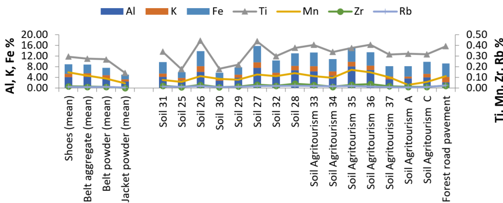
FIGURE 9 Geochemical variability of Fe, K, Al, Ti, Mn, Zr and Rb contents (%) between soil samples collected from items from the victim and reference samples.
