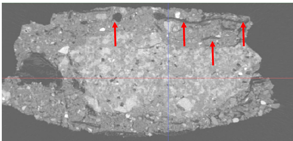
FIGURE 5 X-ray microtomography of the soil aggregate recovered from behind the victim's belt.
