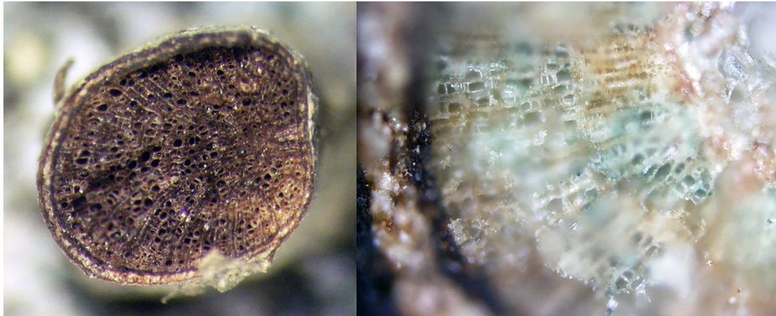
FIGURE 6 Microscopy of plant residues. Left image: Cross-section viewed under a stereomicroscope at 40X magnification. Right image: Cross-section observed under a reflected light microscope at 100X magnification (courtesy of E. Allevato).
