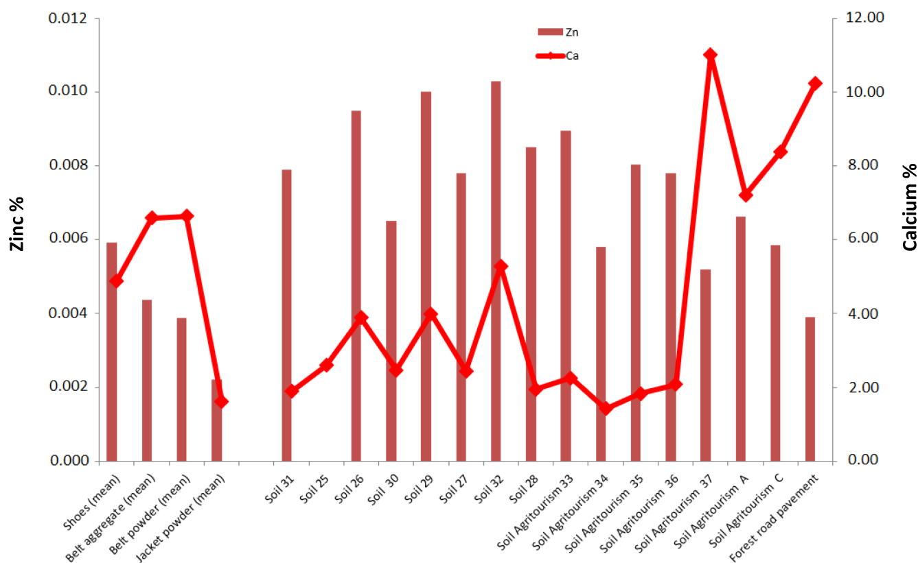
FIGURE 10 Geochemical variability of Ca (ppm) red line and Zn (%) dark red bars.
