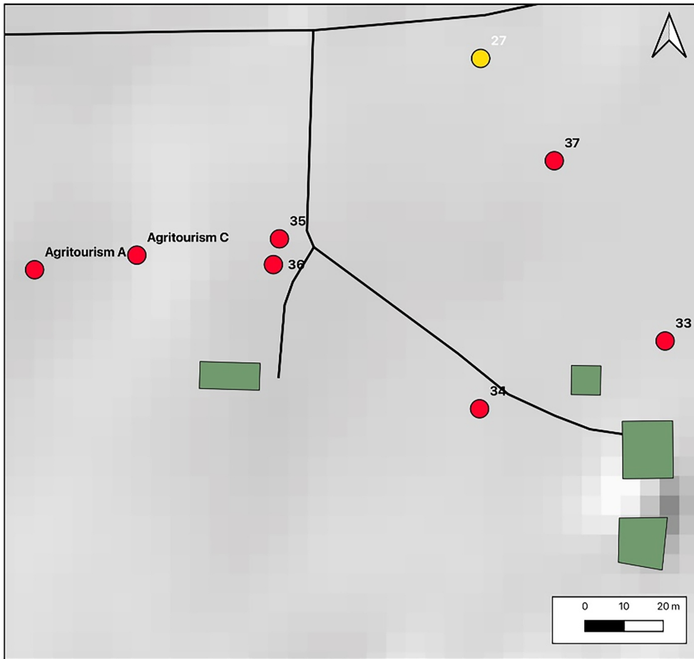
FIGURE 8 Map showing soil sampling points at the Agritourism farm.
