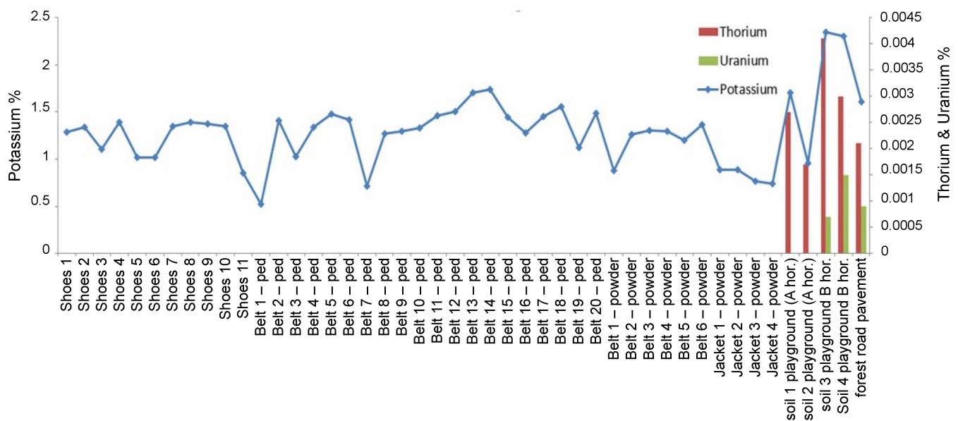
FIGURE 2 Potassium (K) content (%) on the left y-axis and Uranium (U) and Thorium (Th) content (%).
