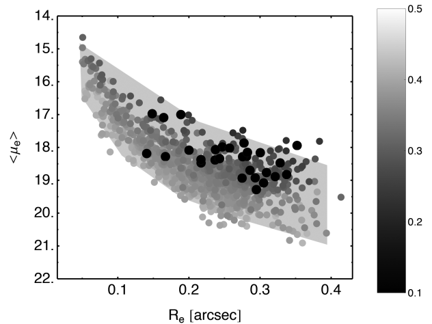
Figure 4. \langle\mu_e\rangle – R_e plane. Small dots are for the UCMG_PHOT sample using MFREE masses and with z_{\text{phot}} \leq 0.5 . The points are colour coded according to their photometric redshift (a colour bar is added to the plot). Larger black dots with grey edges are for all the UCMG candidates in UCMG_NEW. Shaded grey region encloses the 2DPHOT \langle\mu_e\rangle and R_e output values for the mock galaxies simulated in Appendix B. The lower bound of the shaded region corresponds to galaxies with m_S \sim 21 , which is approximately our magnitude limit.
