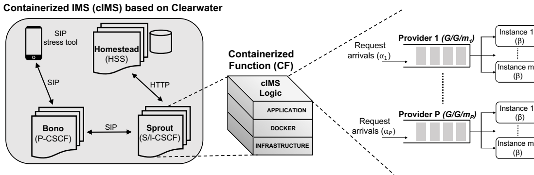
Fig. 1: Architecture overview: the testbed based on the Clearwater platform (left panel); the 3-layer Containerized Function (CF) constituting a cIMS node (middle panel); the G/G/m queueing model for each provider p (right panel).
