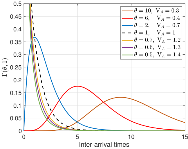
Fig. 7: Gamma-distributed inter-arrival times and corresponding coefficients of variation ( V_A ).
