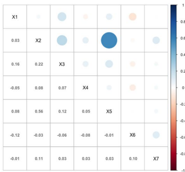
(c) Cluster 3
