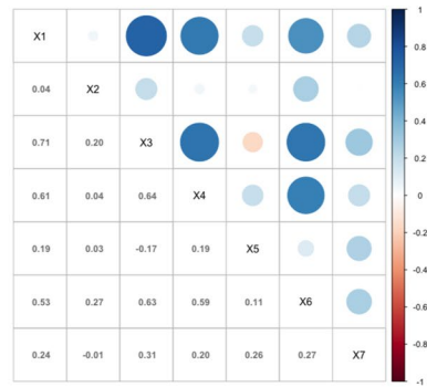
(b) Cluster 2
