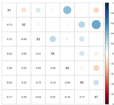
(e) Cluster 5
