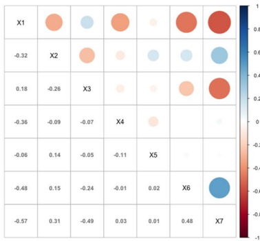
(a) Cluster 1
