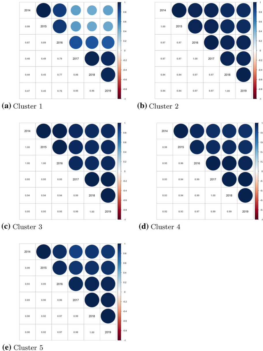
Fig. 2 MMN clusters' corr-plots in time
