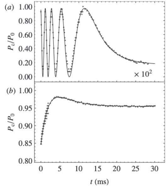
FIG. 3. Time decay of the power of the converted components of the output beam for EOQP 1 (a) and EOQP 2 (b) after the voltage switch-off. The starting voltages were v_1=2.8 V for EOQP 1 and v_2=2.2 V for EOQP 2 so that the dynamics may be approached in the small distortion limit and compared with theory (continuous lines). The time scale in panel (a) is slower by a factor of 100 with respect to panel (b).
