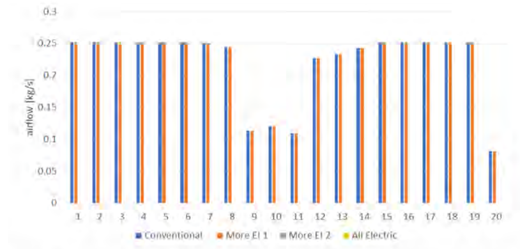
Figure 15. Pneumatic airflow requirement for the four OBS architectures (results from workflow n.4).
