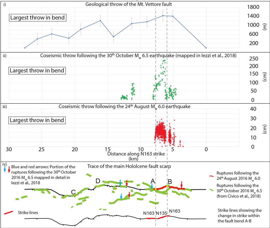
b) Comparison between the geological throw, the coseismic throws and the fault geometry of the Mt. Vettore fault, central Italy (modified from Iezzi et al., 2018)
