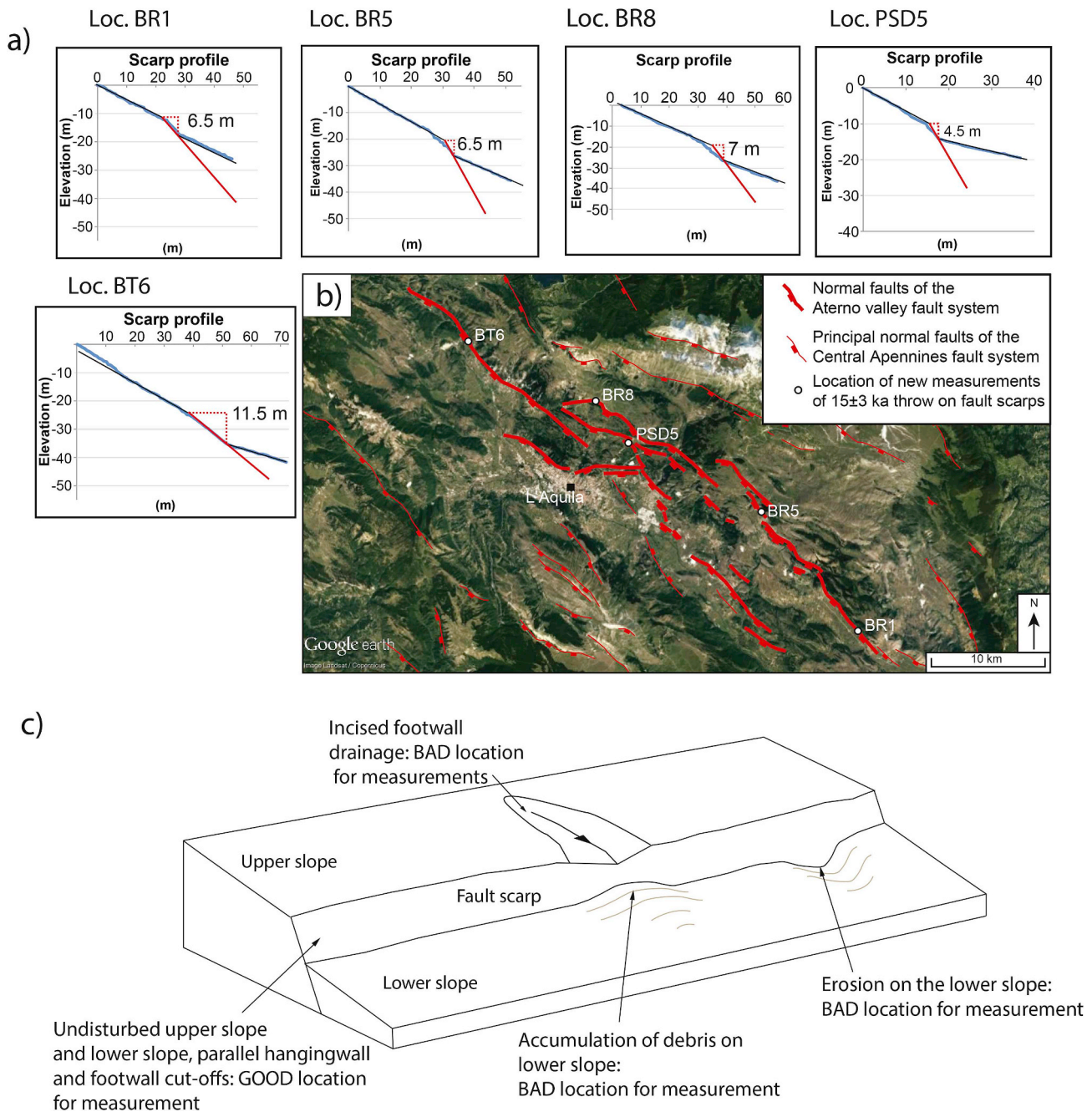
Figure 7. Newly collected field measurements of throw and throw-rates since the demise of the Last Glacial Maximum ( 15 \pm 3 ka) from fault scarps located along the Aterno Valley Fault System. a) Interpreted scarp profiles showing the measured throw associated with the fault scarp. Scarp profiles have been built through chain surveying techniques using a 1 m ruler and a clinometer. Location numbers are coded in agreement with the database shown in Fig. 6b b) Location map of the field locations in a). c) Sketch of a fault scarp to show the criteria we have followed to select the site of measurement. Measurements of scarp height are collected only in locations where upper and lower slopes and hangingwall and footwall cut-offs are preserved since the demise of the LGM ( 15 \pm 3 ka), so to represent the throw accumulated during the last 15 \pm 3 ka.
