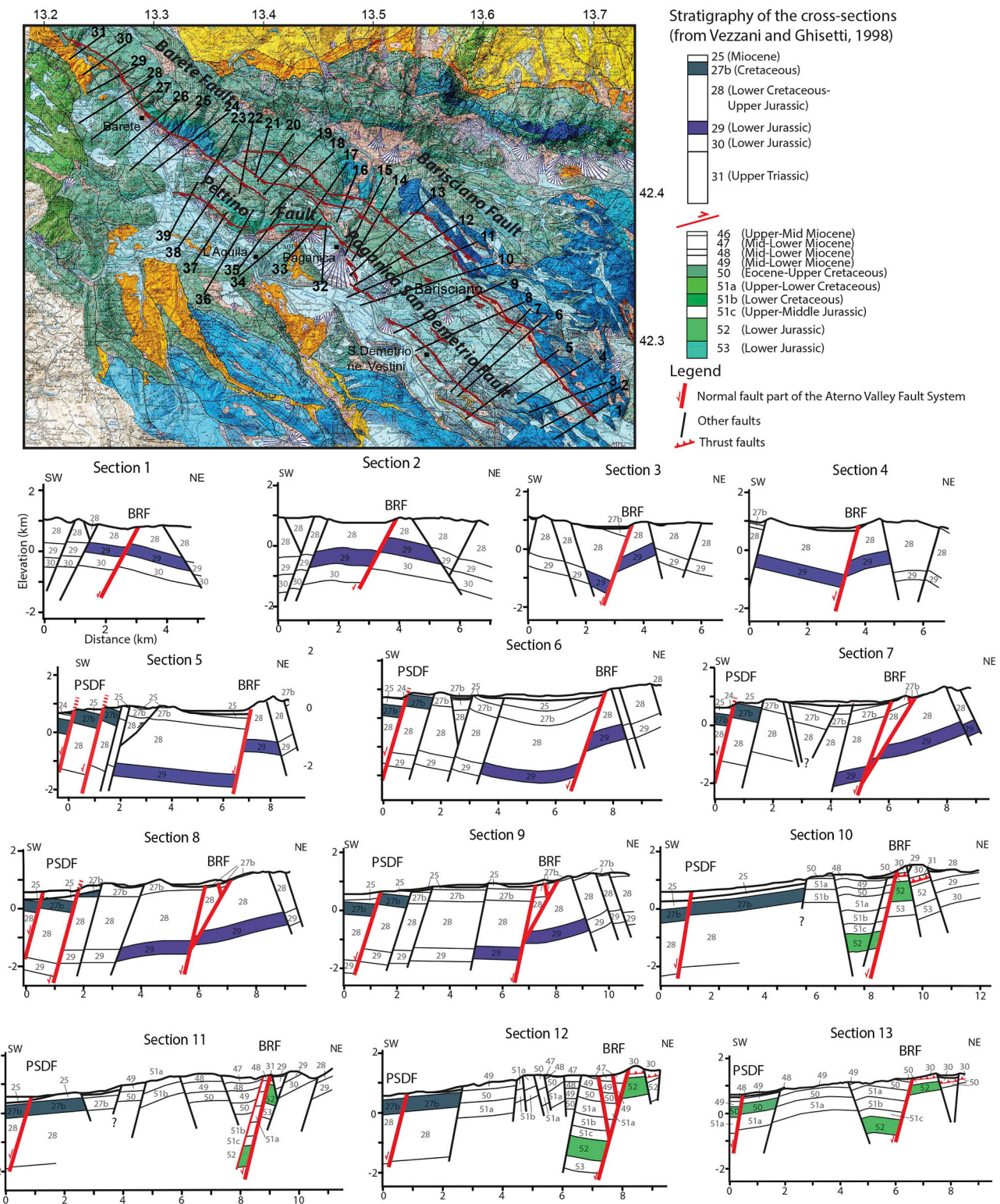
Fig. 5. Geological cross-sections built across the Aterno valley fault system. (a) Geological map of the Aterno Valley Fault System, modified from Vezzani and Ghisetti (1998). Red lines are fault traces of the Aterno Valley Fault System, black lines are traces of the cross-sections. The stratigraphy is derived from Vezzani and Ghisetti, 1998, map; colours are in agreement with the ones reported in the map, and used in the cross-sections to highlight the offset on fault. Here are shown cross-sections from 1 to 13. b) Cross-sections from 14 to 39. BRF: Barisciano fault; PSDF: Paganica-San Demetrio fault; BTF: Barete fault; PF: Pettino fault. When it was not possible to establish the thickness of a formation, we assigned it the maximum thickness provided by the legend of the map.
