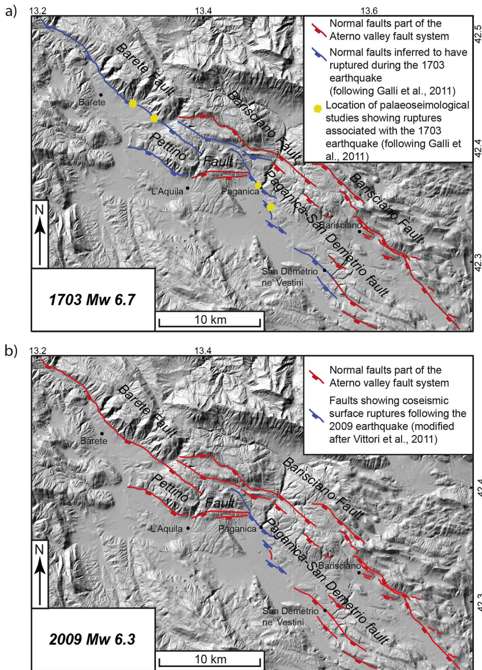
Fig. 4. Palaeoseismological hypothesis of the occurrence of multi-fault earthquakes across the Aterno Valley Fault System. (a) shows in blue fault segments inferred to have ruptured during the 1703 M_w 6.7 earthquake, following Galli et al. (2011). Yellow polygons are locations of palaeoseismological studies with evidences of rupture ascribable to the 1703 earthquake (from Galli et al., 2011). (b) shows in blue surface ruptures following the 6th April 2009 M_w 6.3 earthquake, modified after Vittori et al. (2011). It is shown that palaeoseismological studies suggest that the 1703 M_w 6.7 earthquake have ruptured at the same time several fault segments across the total extension of the fault system, suggesting the occurrence of multi-fault earthquakes.
