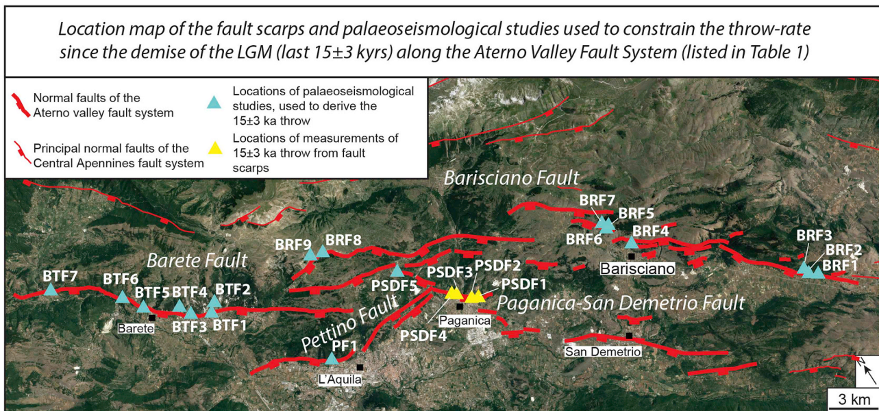
Fig. 6. Location map of the fault scarps and palaeoseismological studies used to constrain the throw rates since the demise of the Last Glacial Maximum ( 15 \pm 3 ka) along the Aterno Valley Fault System, comprehensive of published and newly collected data. Location numbers are coded in agreement with the name of the fault to which they belong: BRF = Barisciano fault; PSDF = Paganica-San Demetrio fault; PF = Pettino fault; BTF = Barete fault.
