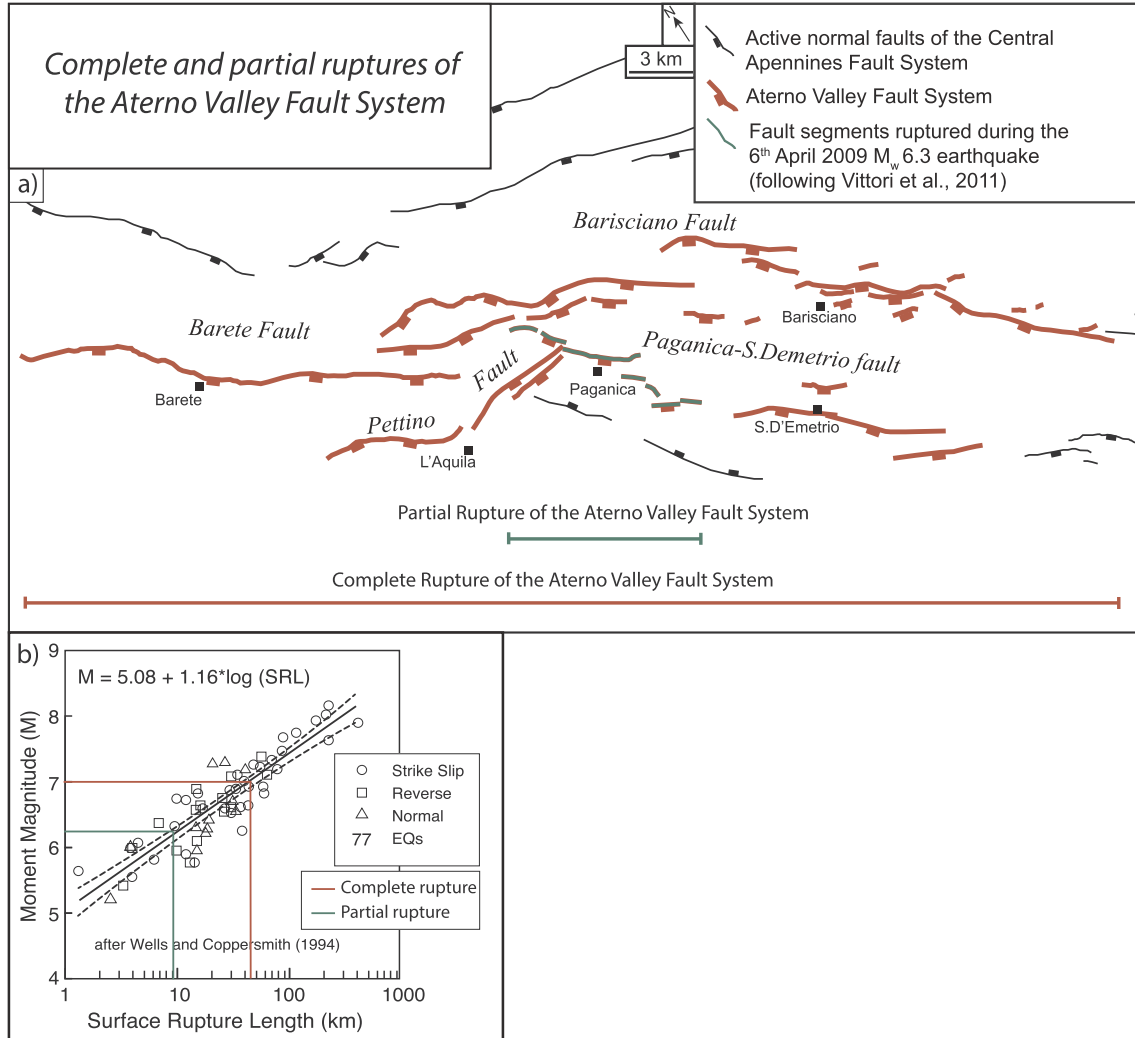
Fig. 11. Complete and partial ruptures of the Aterno Valley Fault System. a) Fault map of the Aterno Valley Fault System showing that it can experience complete ruptures, involving all its fault segments (red bar), and partial ruptures, as is the case of the 2009 M_w 6.3 L'Aquila earthquake (green bar). b) Moment Magnitude versus Surface Rupture Length scaling relationship (Wells and Coppersmith, 1994), with reported partial and total ruptures of the Aterno Valley Fault System.
