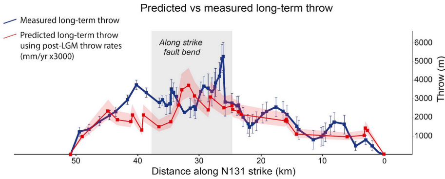
Figure 10. Comparison between the measured long-term throw profile (blue line) and the predicted long-term throw profile (red line), assuming constant post-LGM throw rates since 3 Ma. It shows that the two profiles are overall consistent, which suggest that the post-LGM throw rates can be representative of the throw rates averaged over the entire faults activity. Local discrepancies prompt the idea that post-LGM throw rates are working in order to produce a throw profile which reflect the long-term throw profile.
