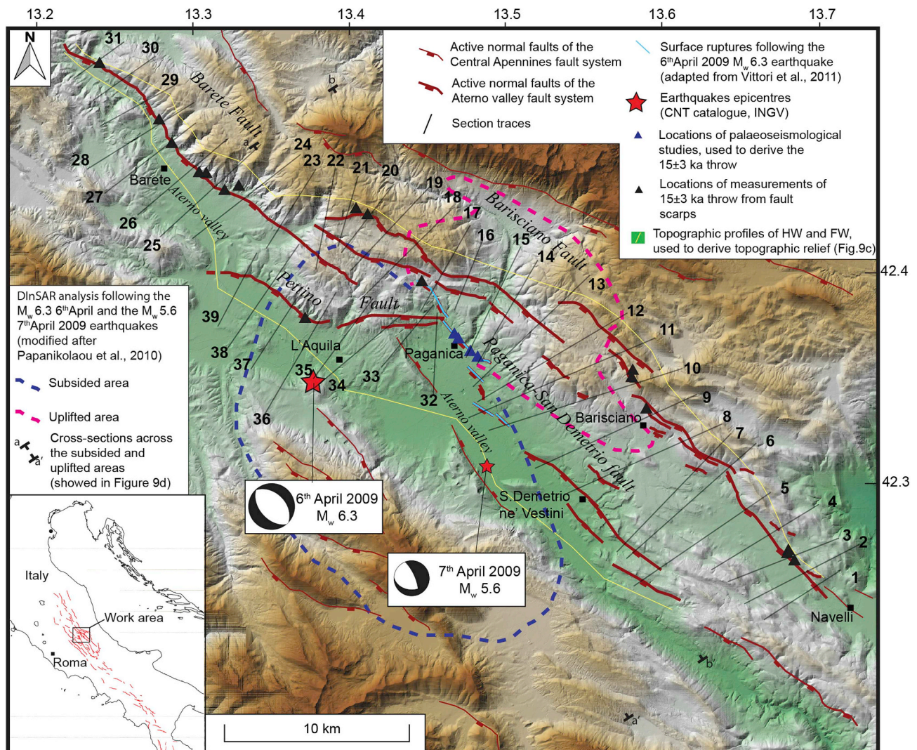
Fig. 2. Location map of the Aterno Valley Fault System, central Apennines, Italy. Thick red lines are normal fault segments part of the Aterno Valley Fault System, thin red lines are other active normal faults part of the Central Apennines Fault System. Black lines are traces of the geological cross sections. Black triangles are locations of measurements of post 15 \pm 3 ka fault throw obtained from fault scarp measurements (from Roberts and Michetti, 2004; Papanikolaou et al., 2005; Galli et al., 2011; our own fieldwork); blue triangles are locations of measurements of post 15 \pm 3 ka fault throw derived from throw rates obtained with palaeoseismological analysis, assuming these throw rates constant within the last 15 \pm 3 ka (from Galli et al., 2010, 2011; Cinti et al., 2011). Red stars are the epicenters of the 6th April 2009 M_w 6.3 L'Aquila earthquake mainshock and of the 7th April 2009 M_w 5.6 aftershock. Pale blue lines are the traces of the coseismic surface ruptures following the 6th April 2009 M_w 6.3 L'Aquila earthquake (modified from Vittori et al., 2011). Blue and pink dashed lines define the areas of subsidence and uplift, respectively, derived from DiNSAR analysis (Papanikolaou et al., 2010). a-a' and b-b' are traces of profiles across the deformed areas (see Fig. 9). Yellow lines are topographic profiles used to derive the topographic relief associated with the Aterno Valley Fault System (shown in Fig. 9c).
