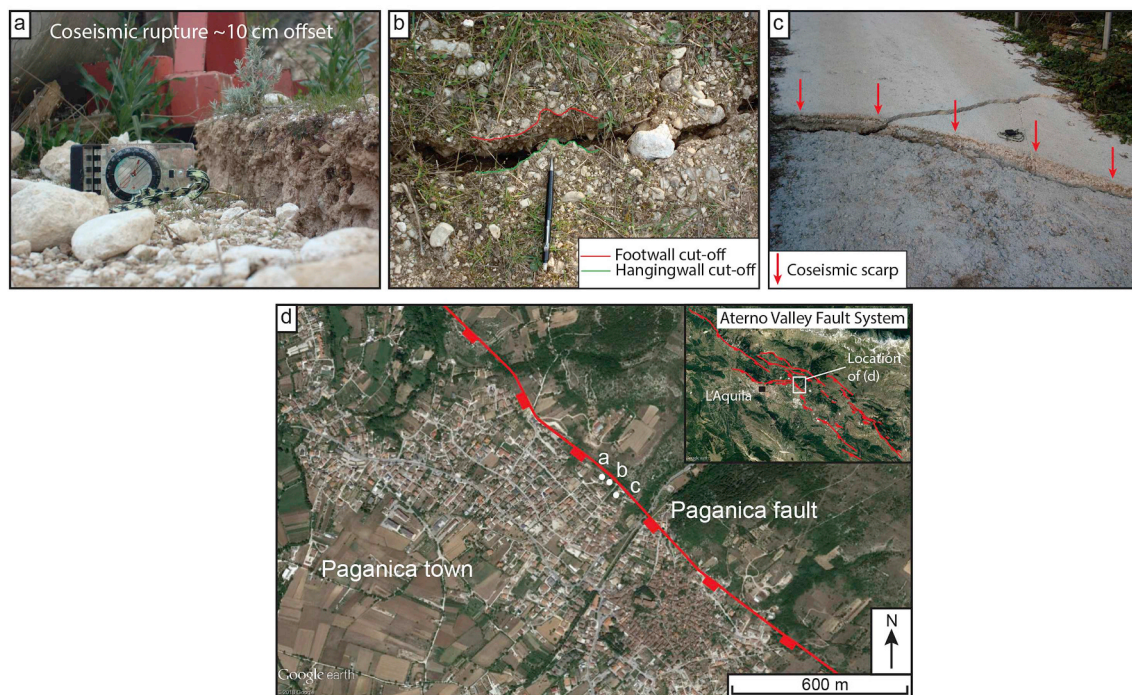
Fig. 3. Coseismic ruptures following the 2009 L'Aquila earthquake. a) Coseismic scarp in eluvial-colluvial deposits, with vertical offset of \sim 10 cm. b) Opening cracks on the ground surface. c) Surface rupture on concrete, with vertical offset of \sim 10 cm. d) Location map of the surface ruptures showed in a), b) and c).
