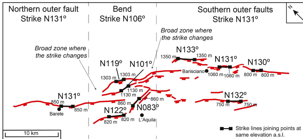
Figure 8. Analysis of the geometry of the Aterno Valley Fault System. In black are reported strike lines built on the main fault segments of the fault system. Strike lines are lines joining locations at the same elevation, and therefore they provide a good representation of the overall strike of the fault segments. It is shown that the fault system presents a wide along-strike bend, across which the strike of different fault segments changes, with an overall shift of \sim 25^\circ from the strike of the fault segments outside the fault bend (outer faults).
