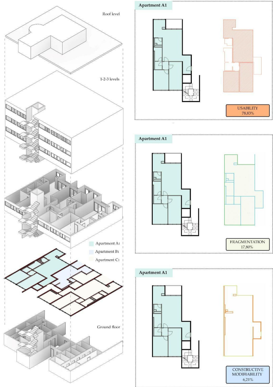
Figure 7. Axonometric cross-section and scores of three indicators.
