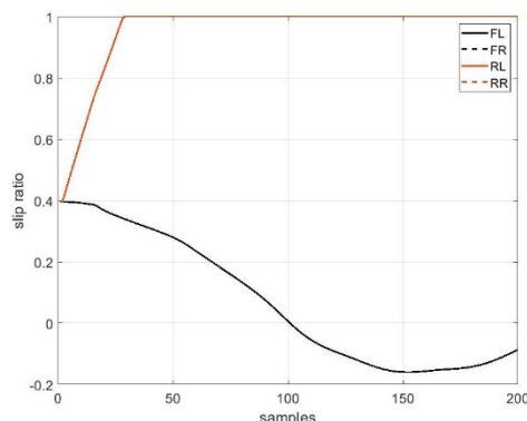
Figure 16. Slip ratio achieved for the four tyres.
