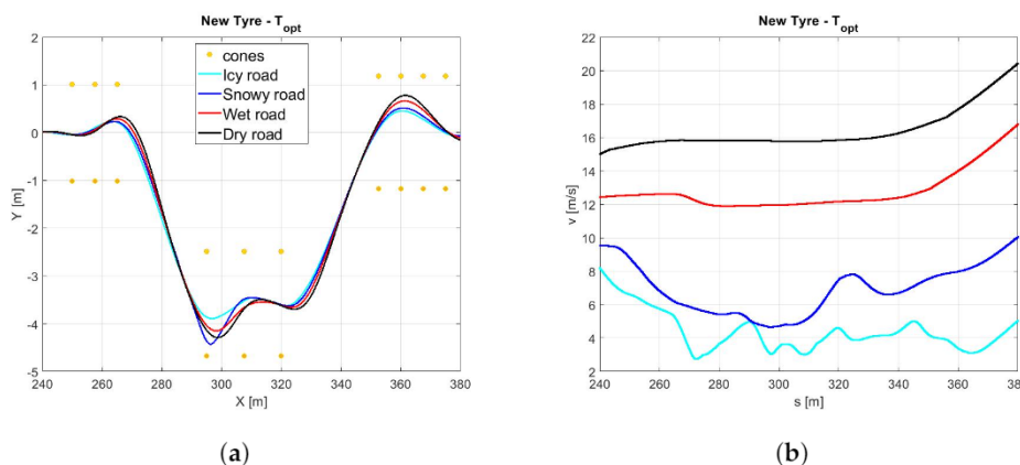
Figure 12. (a) Vehicle trajectory. (b) Vehicle velocity.
