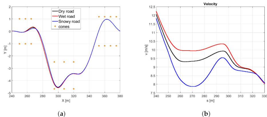
Figure 17. (a) Vehicle trajectory performed in the DLC maneuvers in a dry, wet, and snow road, with new tyre in optimal range temperature. (b) Vehicle velocity
