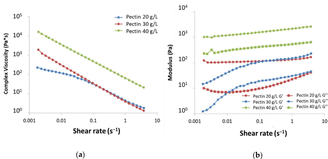
Figure 4. Rheological analysis of pectin gels. (a): complex viscosity ( \eta^* ); (b): storage modulus ( G' ) and loss modulus ( G'' ) vs. shear rate of 20 g/L, 30 g/L, and 40 g/L LM pectin gels.
