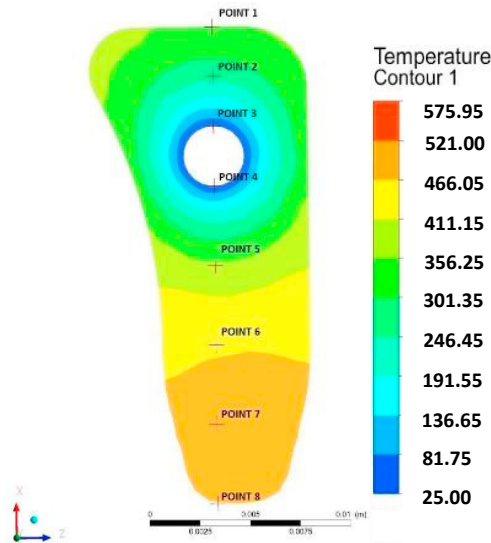
Fig. 6. Temperature in the core of the insert [°C].
