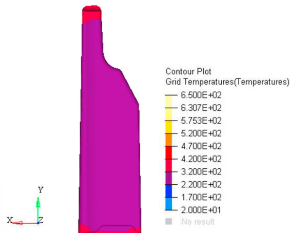
Fig. 13. Temperature field [°C] after 30 seconds.
