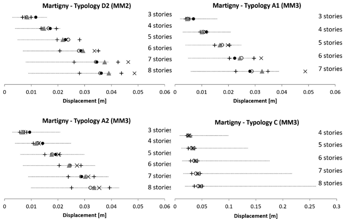
Fig. C2. Displacement demand determination: solid black circle (•) for N2 method; black cross (X) for Lin & Miranda; grey triangle (▲) for N2 OPT) for type D2 compared to the response spectrum of Martigny microzone MM2 and for typologies A1, A2 and C compared to the response spectra of Martigny microzone MM3. The unfilled circles (○) correspond to the average value of the results of NLTHA together with a plus sign (+) for one standard deviation.
