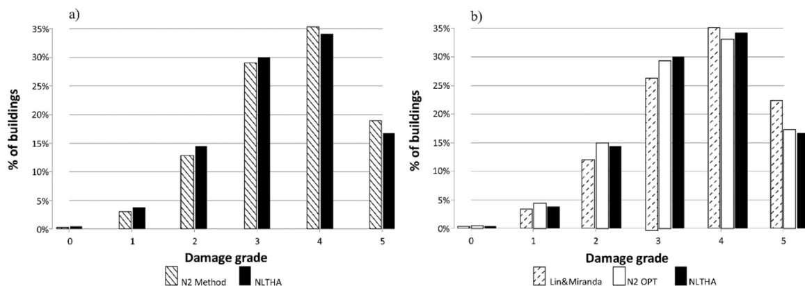
Fig. 13. Damage distribution for Martigny (microzones MM2 and MM3) considering exclusively type D2: N2 method and NLTHA distributions (a.1 and a.2); Lin & Miranda proposal, N2 OPT formula and NLTHA distributions (b.1 and b.2).
