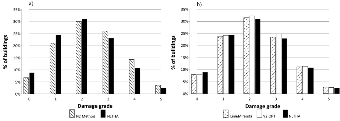
Fig. 8. Damage distribution of Sion (soil C): N2 method and NLTHA distributions (a); Lin & Miranda proposal, N2 OPT formula and NLTHA distributions (b).
