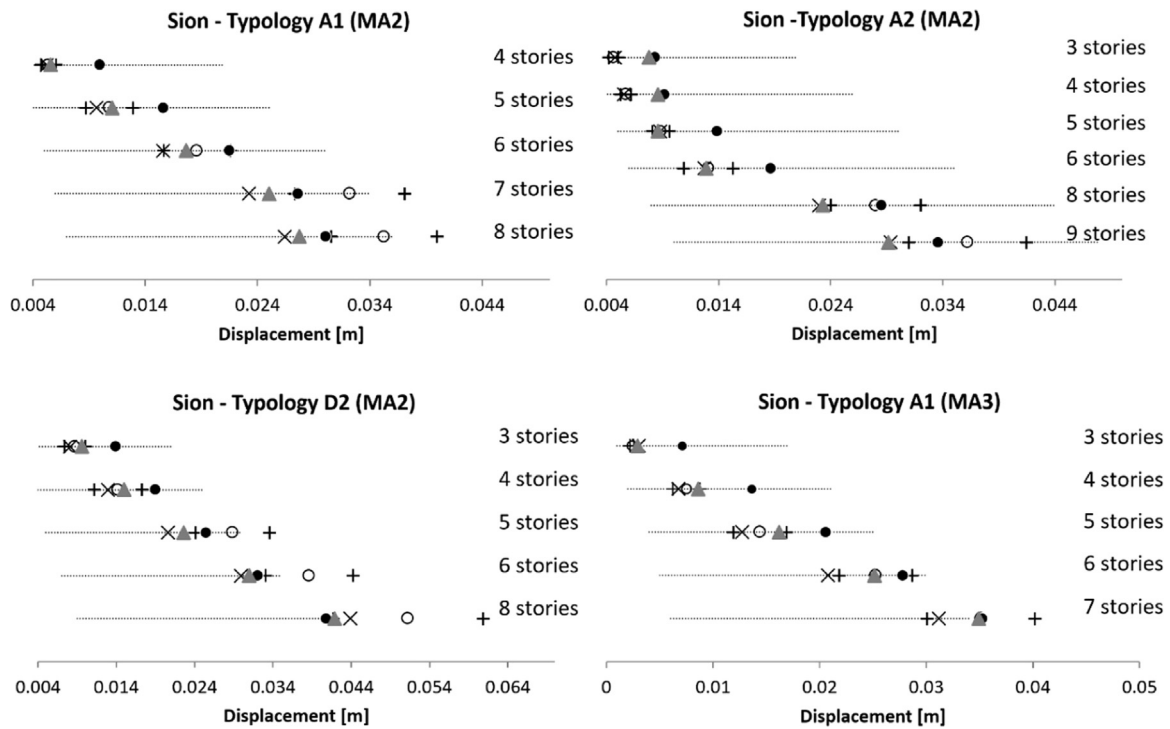
Fig. C1. Displacement demand determination: solid black circle (•) for N2 method; black cross (X) for Lin & Miranda; grey triangle (▲) for N2 OPT) for types A1, A2 and D2 compared to the response spectra of Sion microzone MA2 and for type A1 related to the response spectrum of Sion microzone MA3. The unfilled circles (○) correspond to the average value of the results of NLTHA together with a plus sign (+) for one standard deviation.
