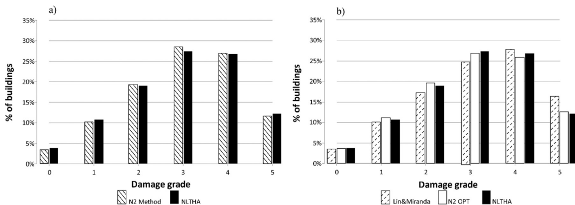
Fig. 12. Damage distribution for Martigny (microzones MM2 and MM3): N2 method and NLTHA distributions (a); Lin & Miranda proposal, N2 OPT formula and NLTHA distributions (b).
