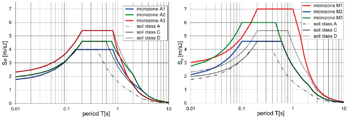
Fig. 10. Elastic response spectra for a return period of 475 years and 5% damping ratio for microzones A1, A2 and A3 of Sion (on the left) and microzones M1, M2 and M3 of Martigny (on the right) (study provided by CREALP).
