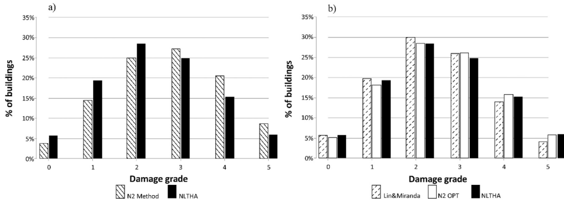
Fig. 11. Damage distribution of Sion (microzones MA1 + MA2 + MA3): N2 method and NLTHA distributions (a); Lin & Miranda proposal, N2 OPT formula and NLTHA distributions (b).
