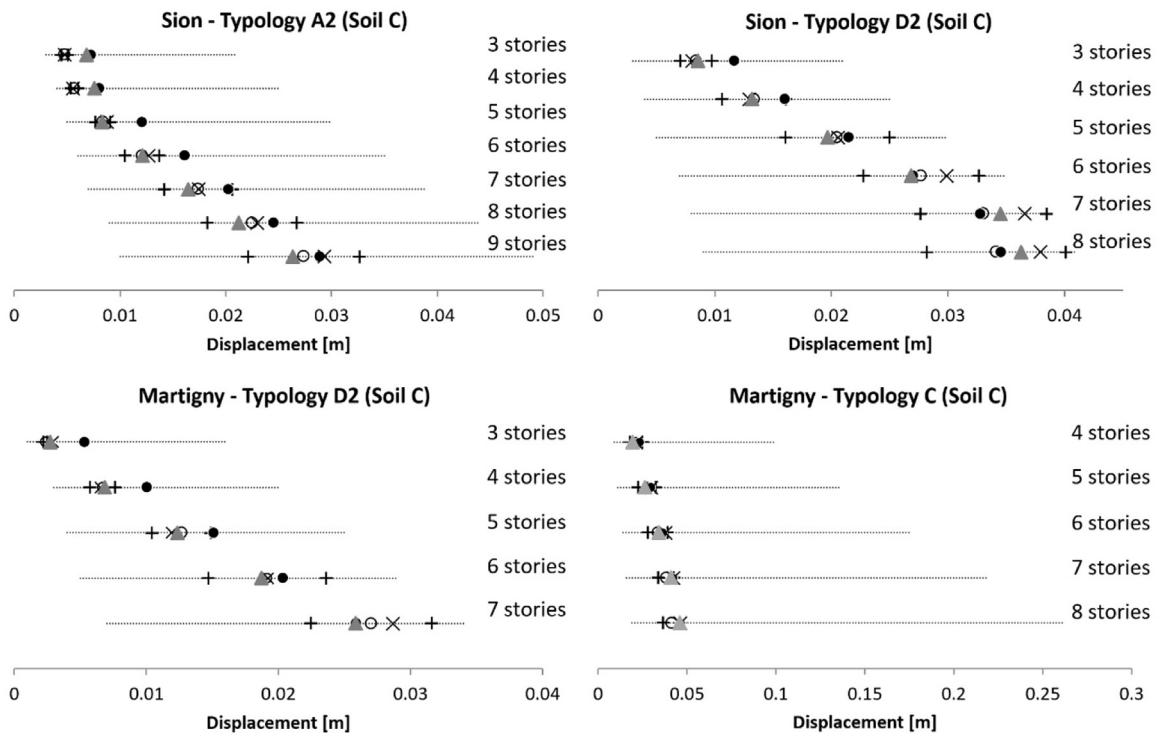
Fig. 7. Displacement demand determination (• = N2 method; X = Lin & Miranda; ▲ = N2 OPT) for types A2 and D2 for Sion and types C and D2 for Martigny for response spectrum of EC8 soil class C and seismic area Z3b. Unfilled circles (○) correspond to the average value of the results of NLTHA together with a plus sign (+) for one standard deviation.
