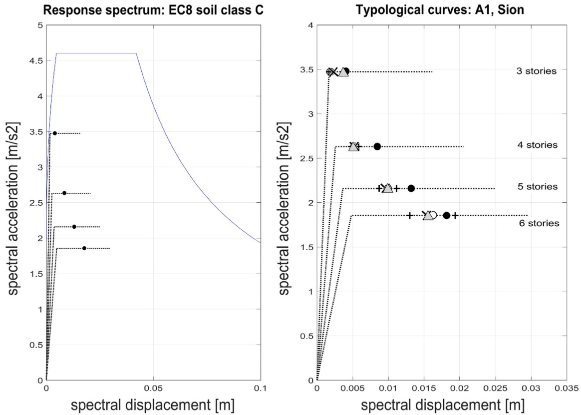
Fig. 6. Typological curves for type A1 in Sion and related performance points (• = N2 method; X = Lin & Miranda; ▲ = N2 OPT) for response spectrum of EC8 soil class C and seismic zone Z3b. Unfilled circles correspond to the average value of the results of NLTHA together with a plus sign for one standard deviation. On the left part of the figure, only performance points obtained by N2 method are shown.
