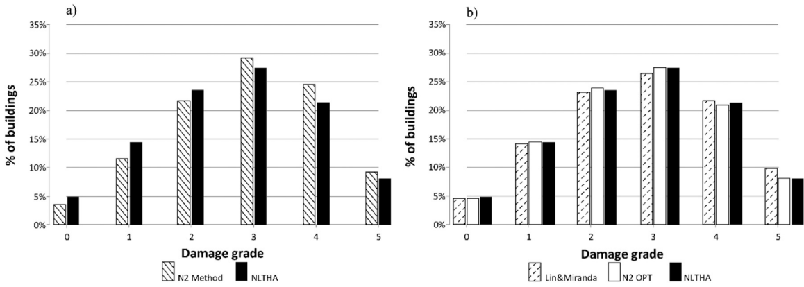
Fig. 9. Damage distribution of Martigny (soil C): N2 method and NLTHA distributions (a); Lin & Miranda proposal, N2 OPT formula and NLTHA distributions (b).
