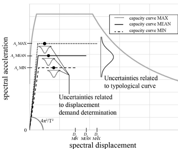
Fig. 5. Uncertainties for the determination of the performance point are related to both the method used for computing the displacement demand and the uncertainties related to the typological curve used.
