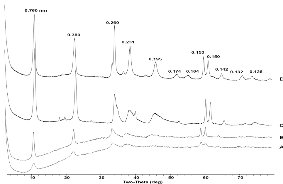
Figure 1. Powder X-ray diffraction patterns of Mg-Fe (A), Cu-Al (B), Mg-Al (C) and Zn-Al (D) layered double hydroxides (modified from Pigna et al. [24]).
