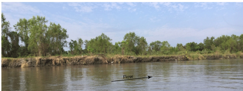
Figure 12. A channel of the Magdalena River close to Barrancabermeja. The land visible here is a macro island vegetated. Along the banks separating the channels from the floodplain, it is common to find dense, tall vegetation (trees); frequent woody debris are indeed present within the channels, often partly or fully buried by sediments.
