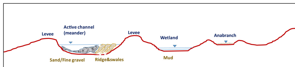
Figure 13. Representative section of a multichannel reach, showing the typical complexity.
