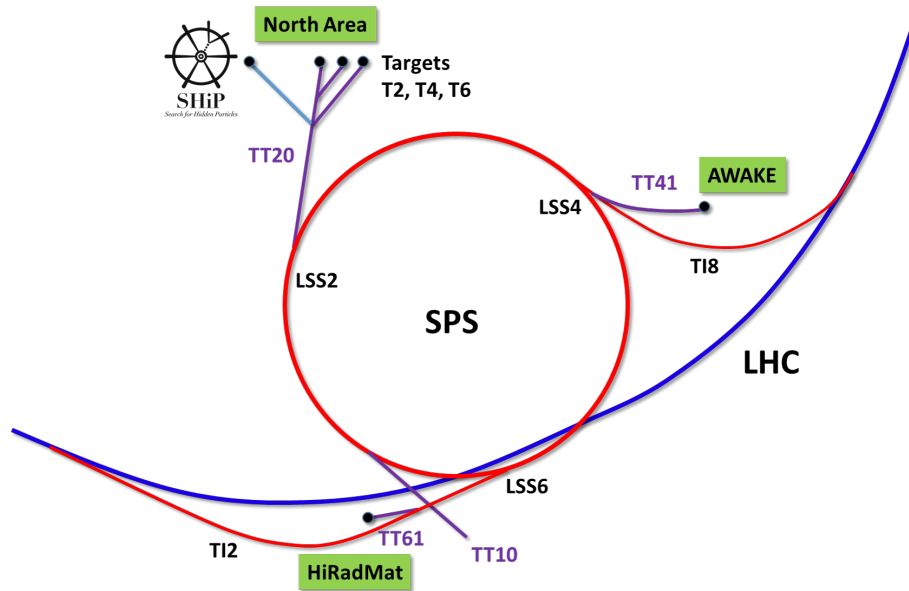
Figure 4. Overview of the SPS accelerator complex. The SHiP experimental facility is located in the North Area and shares the TT20 transfer line with the fixed target programs.
