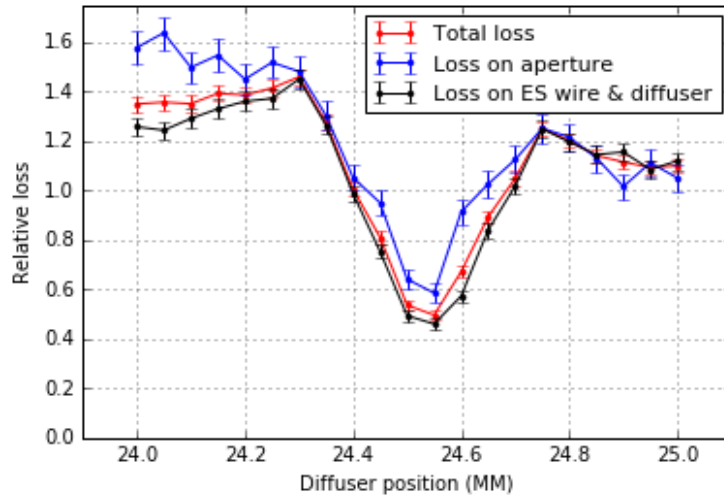
Figure 8. Relative loss of protons in arbitrary units as a function of the transverse position from simulation of a 3 mm long, 0.24 mm wide tungsten-rhenium diffuser. The sum of the loss on the diffuser and the electro-static septum (ES) wires is lower than the total loss with ES wires alone, because the scattering from the diffuser reduces the particle density at the ES sufficiently to result in an overall loss reduction. A factor two improvement is obtained for the optimal position.
