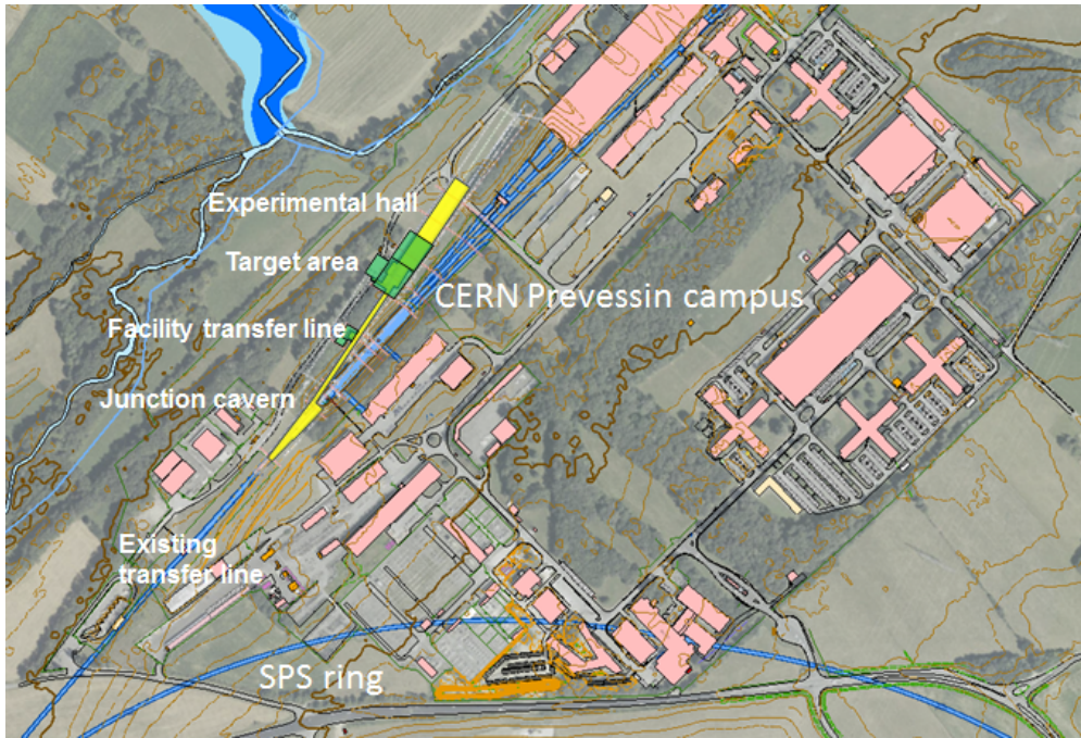
Figure 3. Overview of the required civil engineering for the proposed experimental facility for SHiP on the CERN Preessin campus. The beam-axis is at a depth of about 10 m which allows trenching the entire complex from the surface. New or reworked construction in yellow (underground) and green (surface); existing tunnels in blue.
