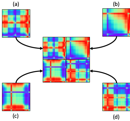
Fig. 2. The policy of composition of the multi-resolution GADF images is shown above; in particular, (a), (b), (c) and (d) refer to the same label, but the observations considered in each are aggregated in four different ways.
