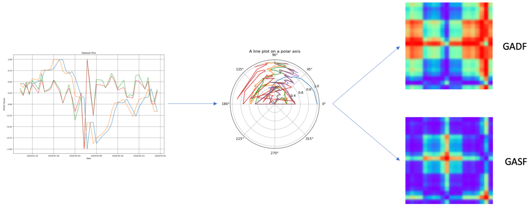
Fig. 1. The figure shows the process leading to the generation of the Gramian Angular Fields images: from left to right, the data are first plotted and then the coordinate system is transformed to a polar plane; finally, the GADF and GASF images are generated according to the function defined in Equation 3.
