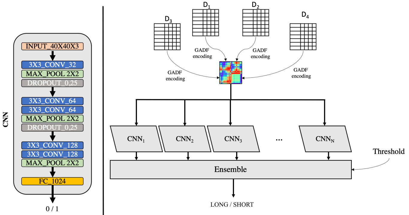
Fig. 3. On the leftmost side of the figure the architecture of the convolutional neural network is shown. On the rightmost side, the overall process of the proposed trading system is depicted.
