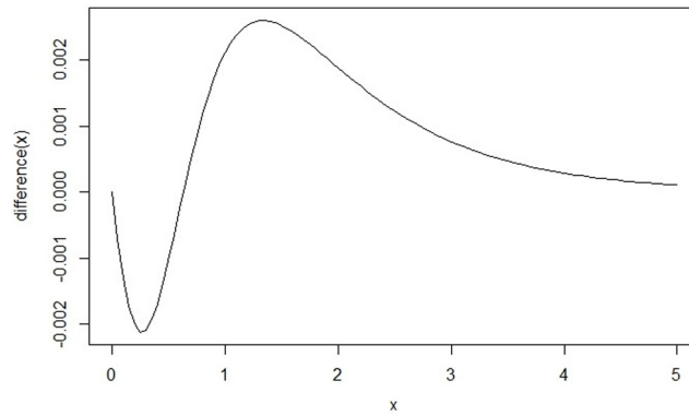
Fig. 1. Plot of the difference \bar{F}_{X_t}(x) - \bar{F}_{\tilde{X}_t}(x) = \bar{F}(x + t, 0)/\bar{F}(t, 0) - \bar{F}(x + t, s)/\bar{F}(t, s) for \bar{F} defined as in (3.1), t = 0.03 and s = 0.06 .
