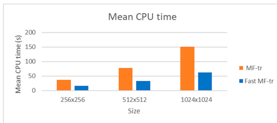
Figure 5. Histogram of the mean CPU times for images with different size.
