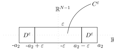
Fig. 2. The set \Omega^\varepsilon = C^\varepsilon \cup D^\varepsilon .
