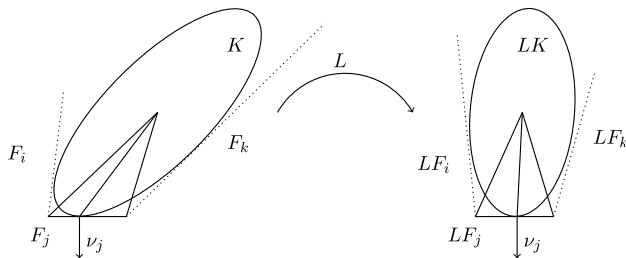
Fig. 1. The linear transformation L .
