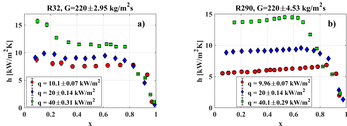
Figure 4. Effect of the heat flux on the mean heat transfer coefficient. The saturation temperature is fixed to 25 °C. (a) R32 with G = 220 \text{ kg}/(\text{m}^2\text{s}) ; (b) R290 with G = 220 \text{ kg}/(\text{m}^2\text{s}) .
