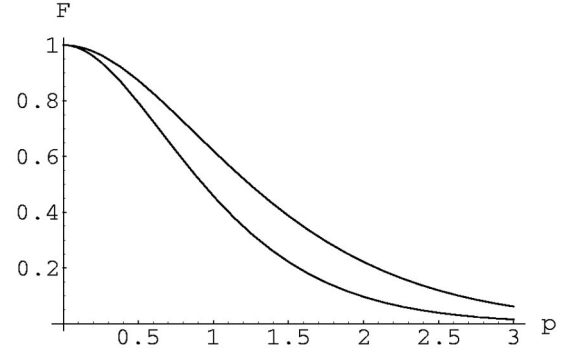
FIG. 3. Form factor F(p) for the D^*D\pi strong coupling as a function of the pion momentum p = |\vec{p}_\pi| in GeV. Normalization is for the soft pion limit. The two curves correspond to \langle k \rangle = 400 MeV (upper) and \langle k \rangle = 300 MeV (lower).
