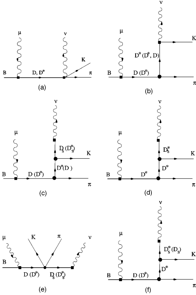
FIG. 2. The relevant Feynman diagrams used to compute T_{\mu\nu} . The box and the circle refer, respectively, to the weak and to the strong interaction. (b) corresponds to three diagrams: the first one has the D state on the horizontal internal line and a D^* state on the vertical line; the second one presents a D^* state on both lines; the third graph has, respectively, a D^* and a D state. The same rule applies to the other figures.
