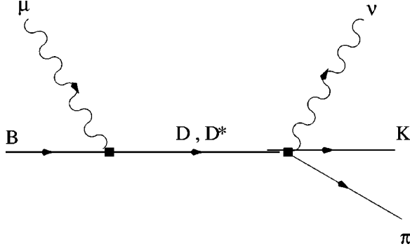
FIG. 1. The diagram corresponding to the hadronic tensor T_{\mu\nu} in Eq. (9). The boxes represent weak couplings.
