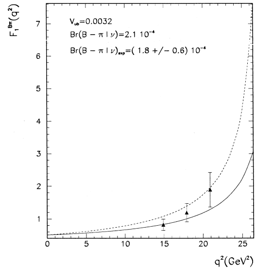
Fig. 1. The semileptonic K \rightarrow \pi , D \rightarrow K , B \rightarrow D and B \rightarrow \pi form factors with, for comparison, a vector dominance, monopole model Eq. (28) and a lattice simulation [23]. Our results: continuous lines. Monopole: dotted lines. Lattice: data points.
