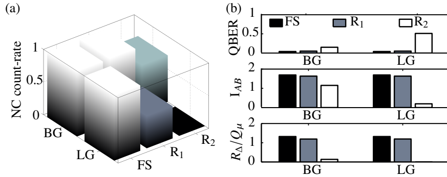
Fig. 6. (a) Experimental normalized coincidence (NC) count-rate for the BG and LG MUB for free-space (FS) and the two obstructions ( R_1 = 600 \mu\text{m} and R_2 = 800 \mu\text{m} ) on the radially polarized mode |\psi\rangle_{00} . (b) The QBER, mutual information ( I_{AB} ) and key rate ( R_{\Delta}/Q_{\mu} ) for the BG and LG modes with no perturbation and under the two tested obstructions are shown.
