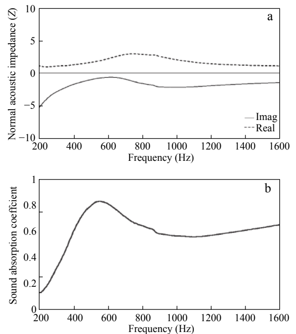
Fig. 11 Acoustic properties of PVP blanket (sample \delta_{1-14} ): real and imaginary parts of acoustic impedance (a) and absorption coefficient (b)
