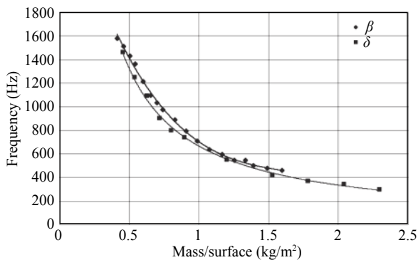
Fig. 10 Plots of the frequency of the sound absorption maximum versus the mass per unit surface of the piled disks
