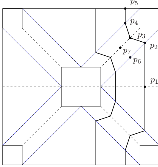
FIGURE 6. A couple of fibers l^m .
