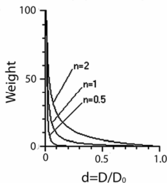
Fig. 9. Curves of the Inverse Distance Weight (IDW).
