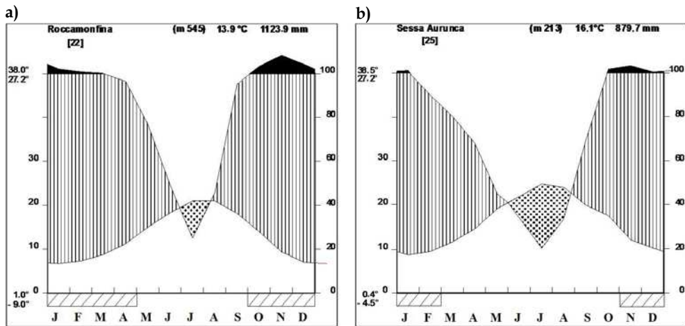
Fig. 6. Thermopluviometric diagrams.
