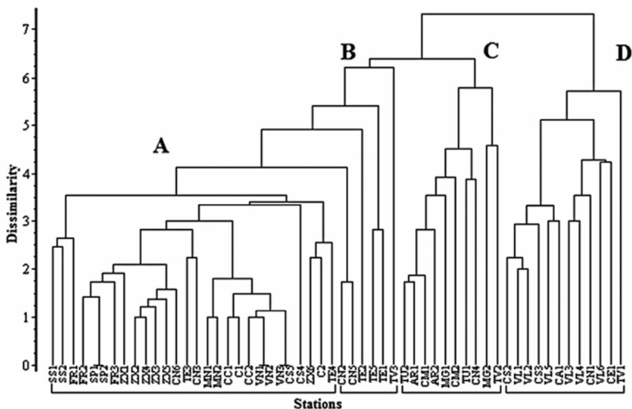
Fig. 14. Dendrogram of the sampling stations. Four clusters (A, B, C, D) resulting by multivariate analysis applied to the sampling stations. See text for details
