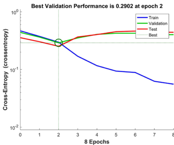
Fig. 16: Best validation performance for ANN
