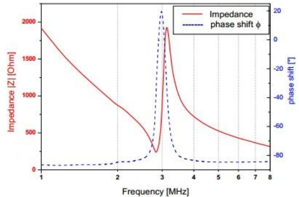
Fig. 5: Resonance phenomena
