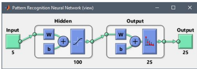
Fig. 15: Neural Network Schematic Form in MatLab 2016
