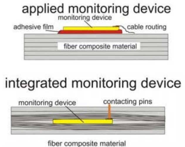
Fig. 6: Applied (up) and integrated (down) device comparison
