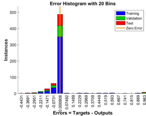
Fig. 17: Histogram Error for ANN Training
