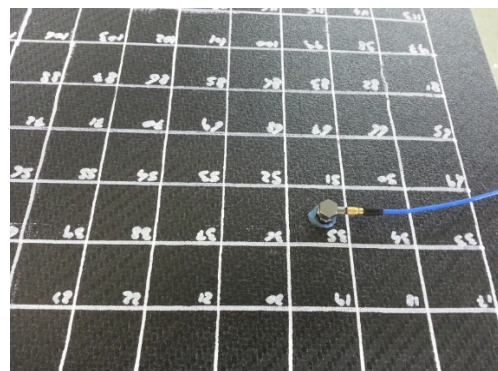
Fig. 3: Detail of Panel and accelerometer
