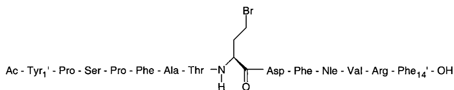
Fig. 6. Sequence of peptide Br-PID. The bromo-homoalanine reacts with the cysteine 30 of the active site to form a thioether bond.
