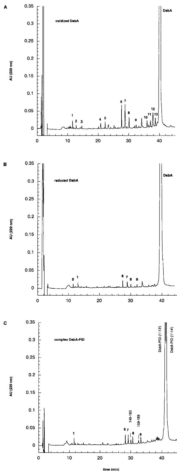
Fig. 4. Comparative HPLC profiles of the tryptic digests of (A) oxidized DsbA, (B) reduced DsbA, and (C) complex DsbA-PID after 60 min incubation using an enzyme/substrate ratio of 1 : 70. Individual fractions were collected and analyzed by ES/MS.
