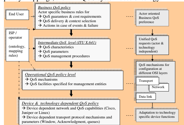
Fig. 2. Hierarchical NETQOS framework for heterogeneous Internet
