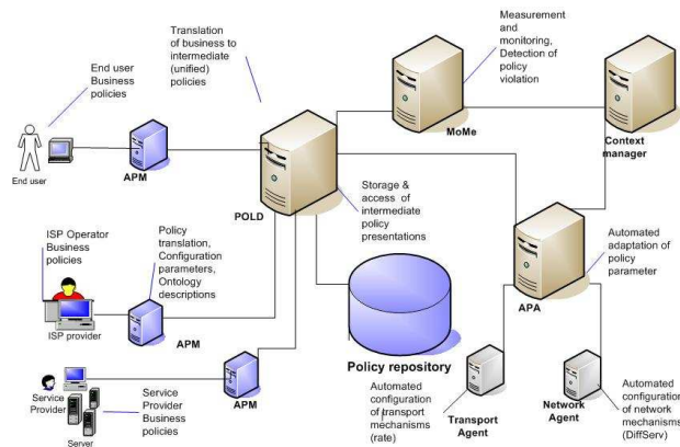
Fig. 1. Interaction of components in the NETQOS architecture
