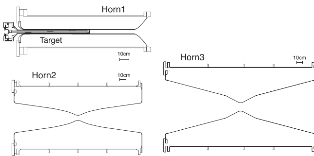
FIG. 6. Cross section view of horns.
