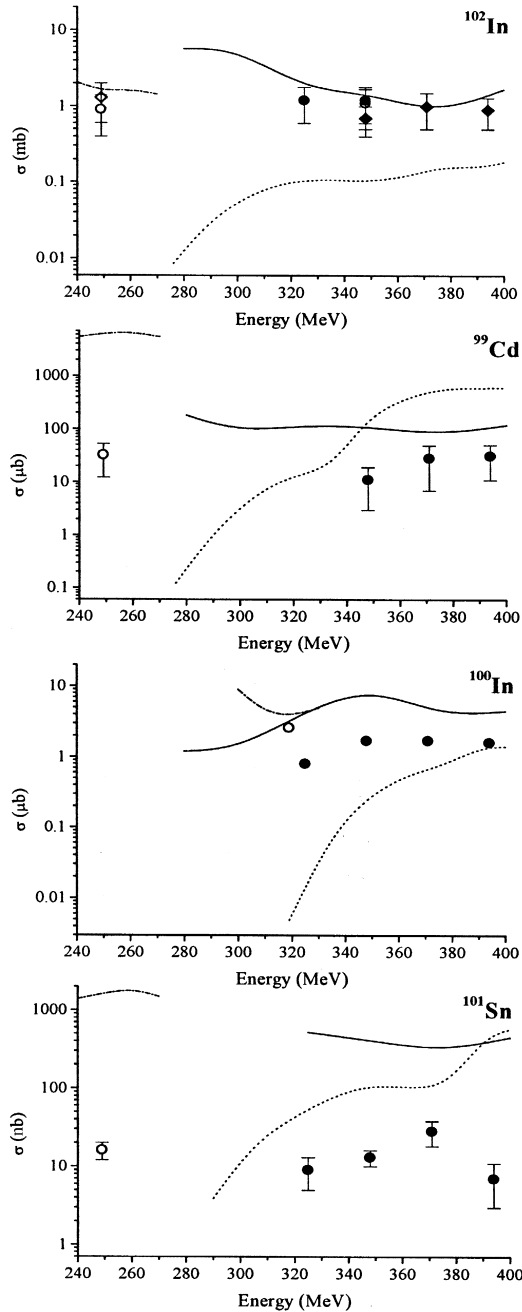
Fig. 2. Experimental and calculated \sigma values as a function of the ^{58}\text{Ni} -beam energy in the middle of targets. The data for the ^{58}\text{Ni} + ^{50}\text{Cr} reaction (open circles) and the ^{58}\text{Ni} + ^{58}\text{Ni} one (solid circles) were deduced from \beta\text{p} activities; for ^{102}\text{In} further data were deduced from \beta\gamma activity for the ^{58}\text{Ni} + ^{50}\text{Cr} reaction (open diamonds) and for the ^{58}\text{Ni} + ^{58}\text{Ni} one (solid diamonds). The data for ^{100}\text{In} represent upper limits. The calculations represent HIVAP predictions for the ^{58}\text{Ni} + ^{50}\text{Cr} reaction (dash-dotted line) and for the ^{58}\text{Ni} + ^{58}\text{Ni} one (dotted line), and BUSCO predictions for ^{58}\text{Ni} + ^{58}\text{Ni} reaction (solid line).
