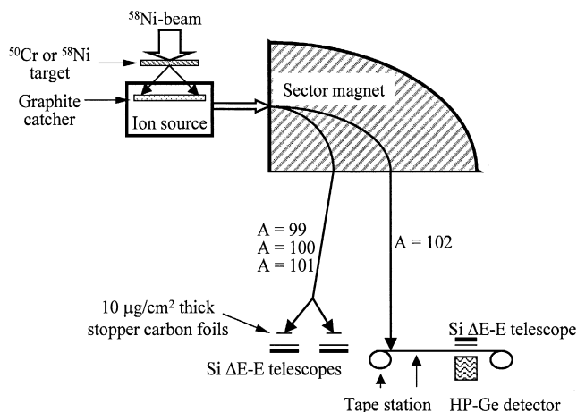
Fig. 1. Outline of the experimental set-up (see text for details).
