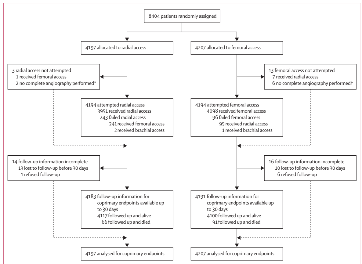
Figure 1: Trial profile
