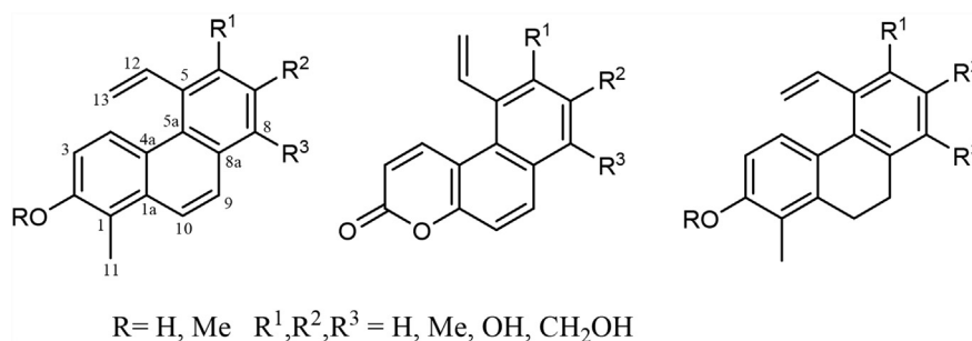
Figure 2. Structure of phenanthrene, benzocoumarin and 9,10-dihydrophenanthrene.
