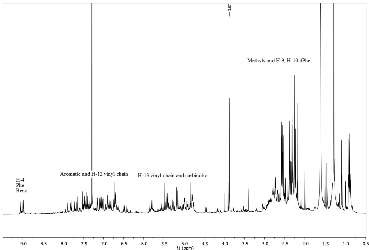
Figure 1. ^1\text{H} NMR of J. acutus active fraction.
