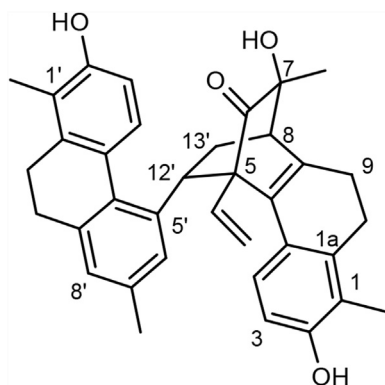
Figure 3. Structure of dimeric 9,10-dihydrophenanthrene.
