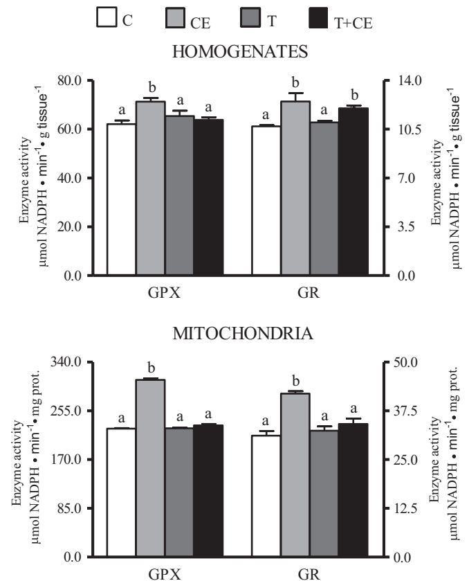
Fig. 5. Antioxidants enzyme activity in liver homogenates (upper panel) and mitochondria (bottom panel) from C, control; CE, cold exposed; T, cold trained; T+CE, cold trained and cold exposed rats. Values are means \pm S.E.M. For each value eight rats were used. Glutathione peroxidase activity (GPX) is expressed in \mu\text{mol NADPH min}^{-1} per g tissue. Glutathione reductase (GR) is expressed in \mu\text{mol NADPH min}^{-1} per g tissue. Different letters indicate significant differences ( P < 0.05 ) between groups. Significant effect of cold exposure ( P=0.0236 ), and interaction between factors ( P=0.0025 ) on homogenate GPX. Significant effect of cold exposure ( P=0.0002 ) on homogenate GR. Significant effect of cold exposure ( P=0.0001 ), cold training ( P=0.0001 ), and interaction between factors ( P=0.0001 ) on mitochondrial GPX. Significant effect of cold exposure ( P=0.0001 ), cold training ( P=0.0069 ), and interaction between treatments ( P=0.0003 ) on mitochondrial GR.
