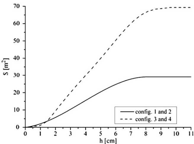
Fig. 3. Stage-area curves.
