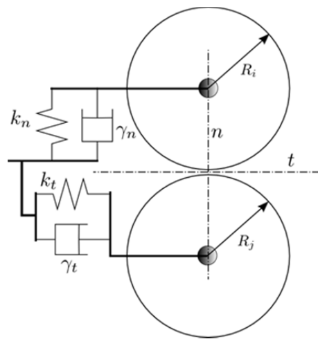
Figure 1. Spring–dashpot contact model.
