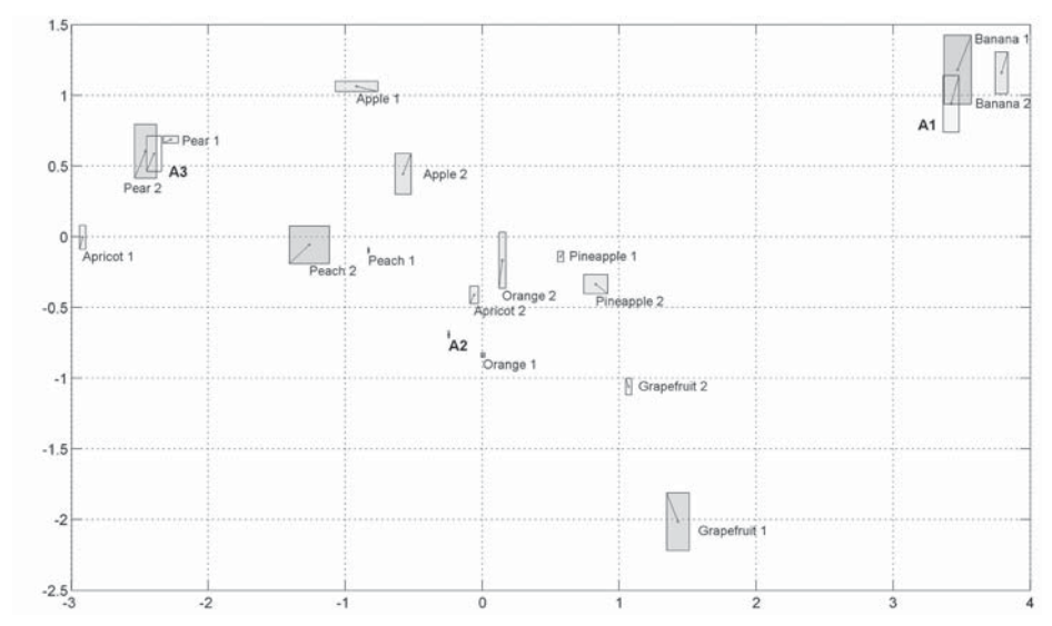
Fig. 3: Archetypes and original statistical units over the first PCA factorial plan.
