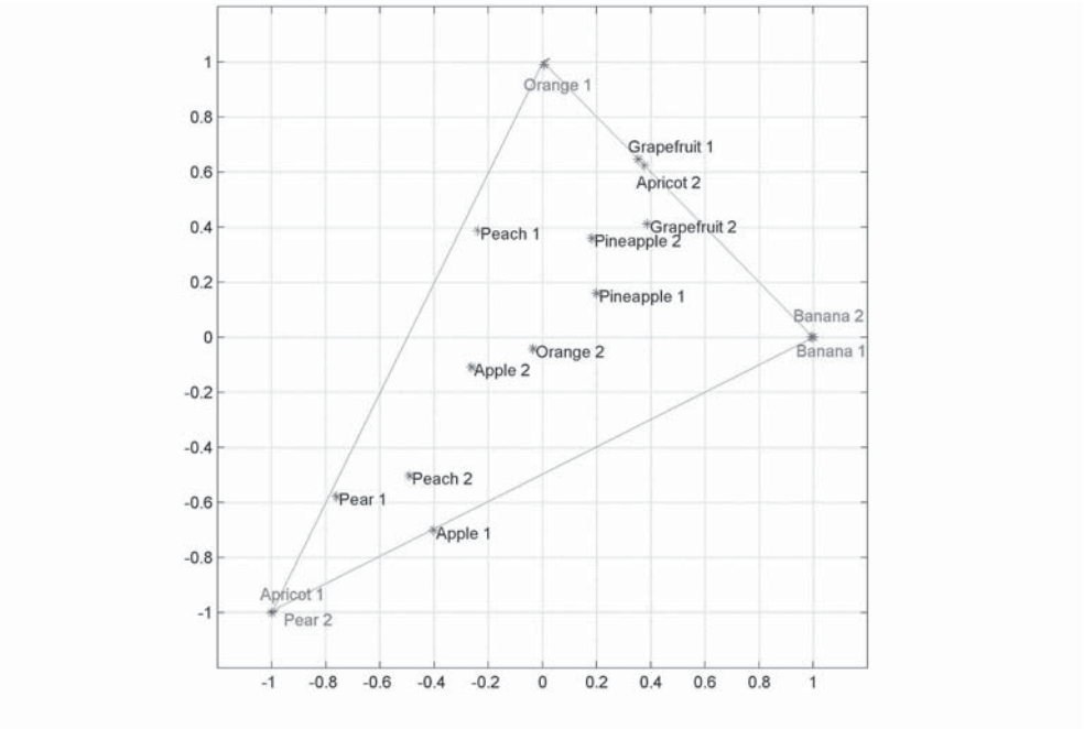
Fig. 2: Plot of the observed data using as coordinates the \alpha'_i coefficients for the Juices dataset for m = 3 archetypes.
