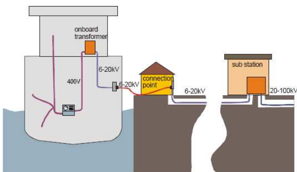
Figure 1. Scheme of cold ironing connection
