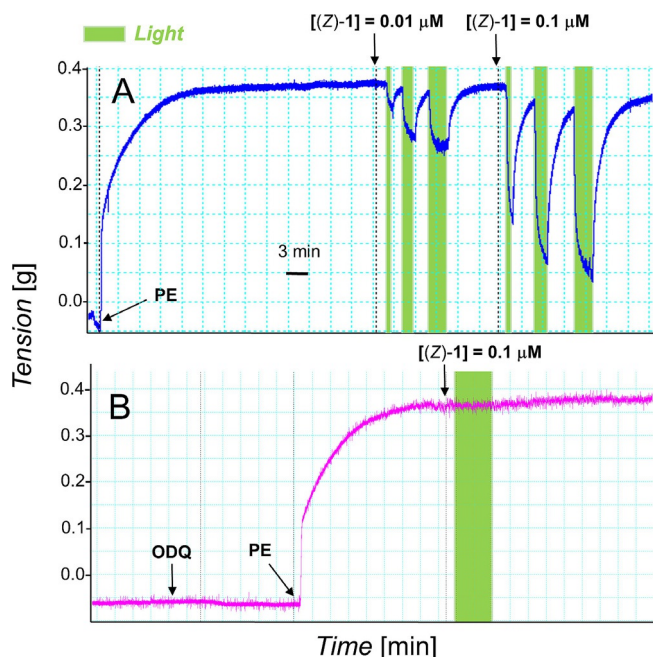
Figure 4. A) Changes in tension of rat aorta induced by NO release from (Z)-1 upon 1, 2, and 3 min irradiation with visible light (515–565 nm, 6.5 \text{mWcm}^{-2} ). B) Control experiment performed by pre-treating the aorta strips with ODQ (10 \mu\text{M} ) before the addition of PE (1 \mu\text{M} ) and (Z)-1, effectively inhibiting NO uptake.
