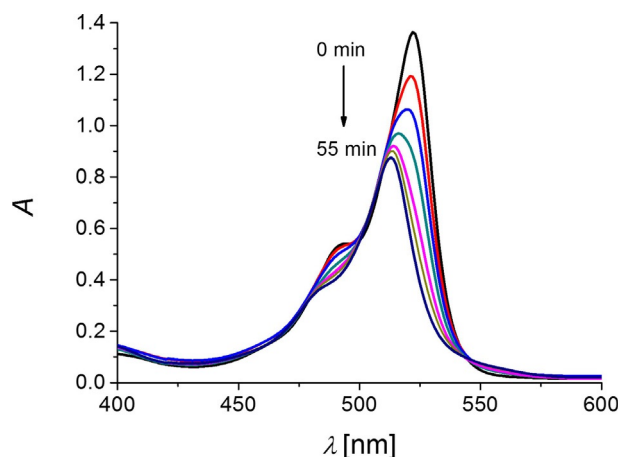
Figure 1. Absorption spectral changes observed upon exposure of a PBS:MeOH (1:1 v/v) solution of (Z)-1 (20 μM) to \lambda_{\text{exc}}=532 nm light for intervals of 0, 5, 10, 15, 25, 35, and 55 min. T=25^\circ\text{C} .
