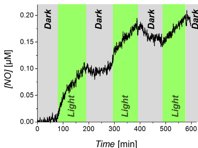
Figure 3. NO release profile observed upon 532 nm light irradiation of a PBS/MeOH (1:1 v/v) solution of (Z)-1 (20 \mu\text{M} ).
