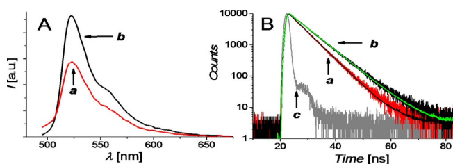
Figure 2. A) Fluorescence emission spectra of optically matched PBS:MeOH (1:1 v/v) solutions of (Z)-1 (a) and 2 (b) at \lambda_{\text{exc}}=480 nm. B) Fluorescence decay and related biexponential fitting of the same solutions as (A) recorded at \lambda_{\text{exc}}=455 nm and \lambda_{\text{em}}=525 nm. C) The instrumental response is also shown.
