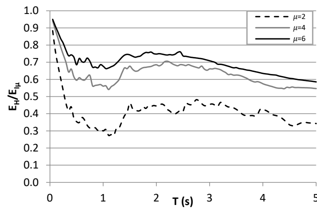
Figure 19. Average spectra of E_H/E_{I\mu} for hysteric model = elasto-elastic, with ductility factors \mu = 2 , \mu = 4 and \mu = 6 , an aftershock magnitude of \gamma = 1.0 and a damping coefficient of \zeta = 5\% .
