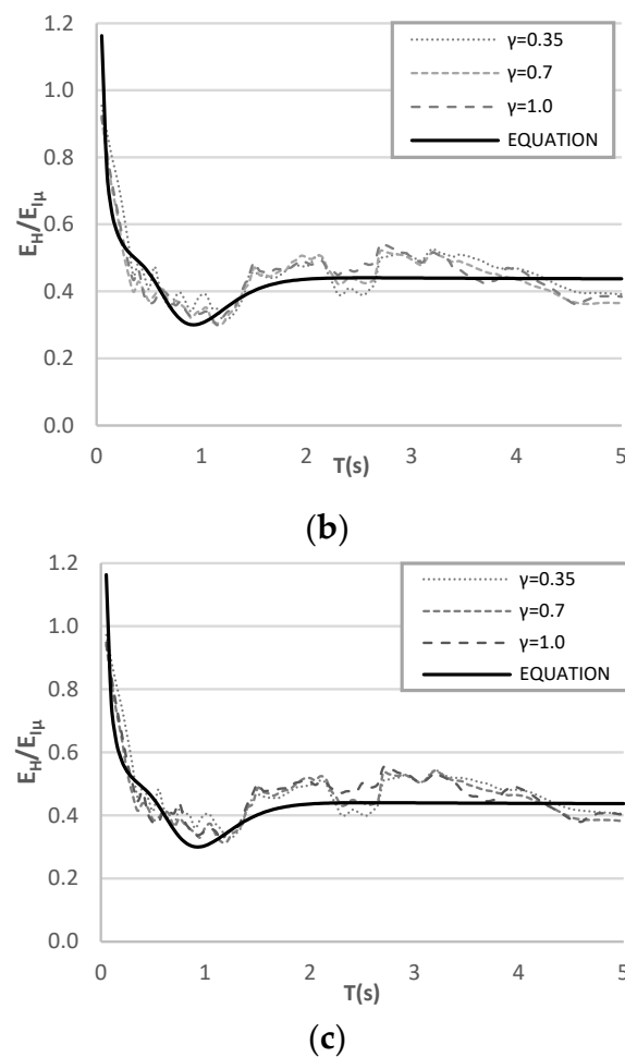
Figure 22. Comparison of the average spectra of E_H/E_{I\mu} for the aftershock magnitudes of \gamma = 0.35 , \gamma = 0.7 and \gamma = 1.0 and spectra of E_H/E_{I\mu} of the proposed Equation (5), with a ductility of \mu = 2 , a damping coefficient of \zeta = 5\% and the hysteric models: (a) elastoplastic, (b) bilinear 3% and (c) bilinear 5%.
