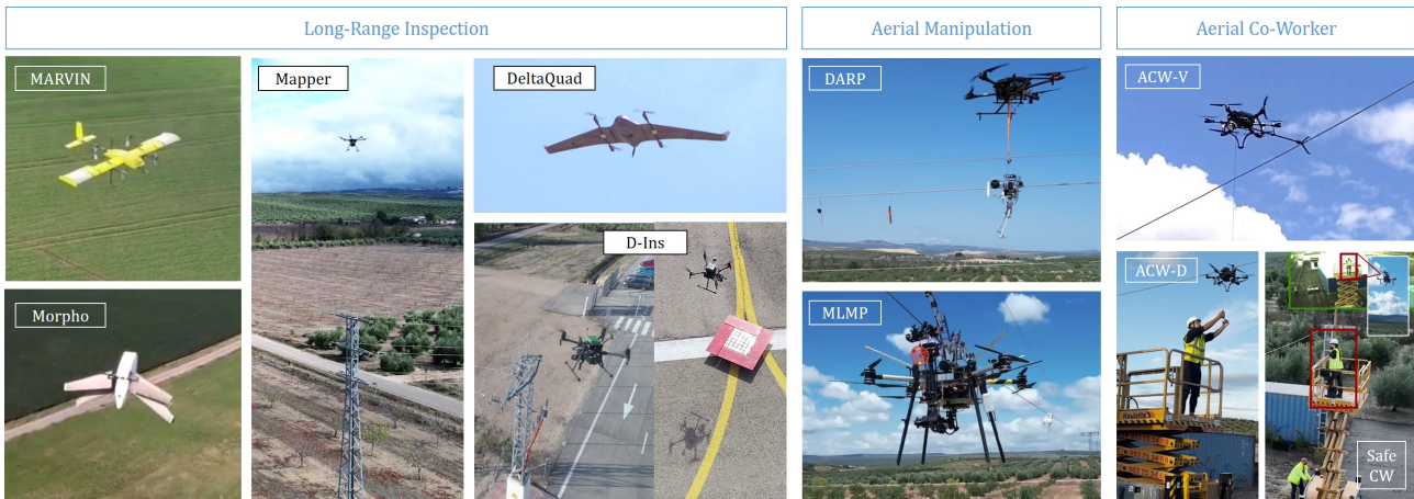
Figure 2: Aerial robotic platforms in the AERIAL-CORE final demonstrations, organized according to the operation domains.
