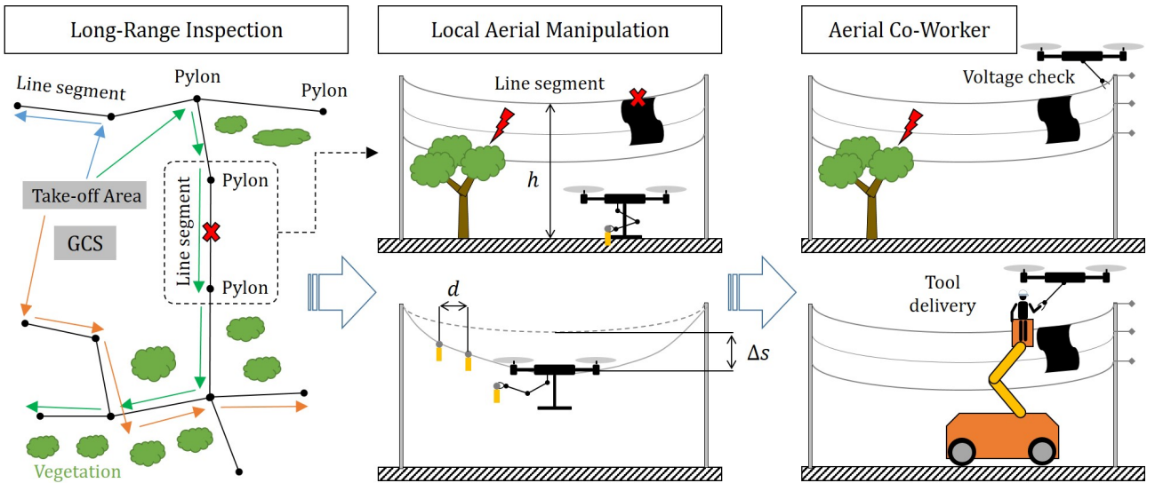
Figure 3: The three operation domains considered in the validation scenario: Long-Range Inspection (left), Local Aerial Manipulation (center), Aerial Co-Worker (right).
