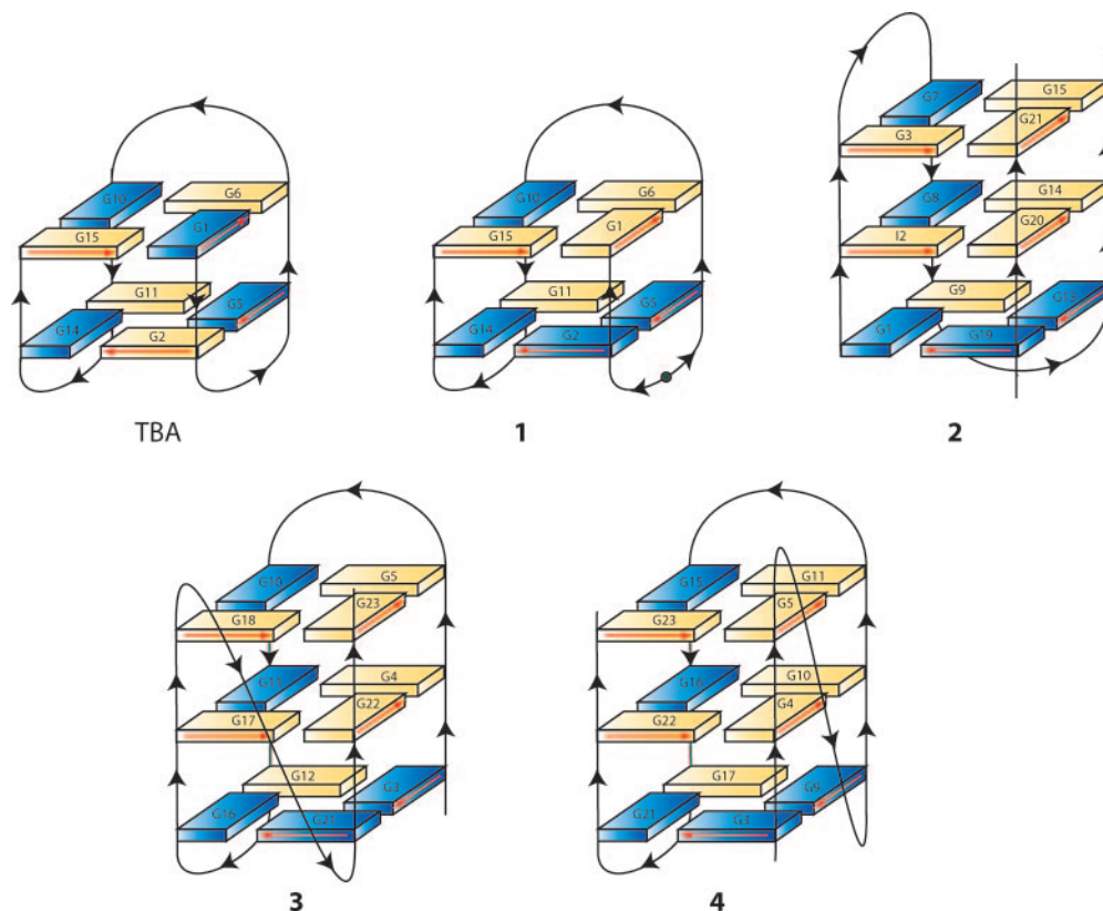
Figure 1. Schematic illustration of the structures adopted by TBA, modified TBA (1), the three human telomeric repeats sequence into a dimeric quadruplex (22) (2), the four-repeat Tetrahymena d(T 2 G 4 ) 4 sequence (23) (3), and the four-repeat human telomeric d[TAGGG(TTAGGG) 3 ] sequence in K + solution (24,25). Black arrowheads indicate 5'→3' polarity of the strands. Black circle in 1 represents the 5'-5' inversion of polarity site. Anti and syn guanines are depicted as yellow and blue solids, respectively. Red arrows indicate the direction of the proton donors and acceptors in Hoogsteen hydrogen bonds.
