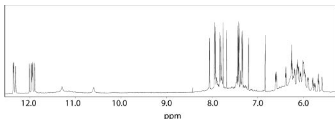
Figure 2. Expanded region of the proton NMR spectrum of 1 (700 MHz, T = 25^\circ\text{C} ).
