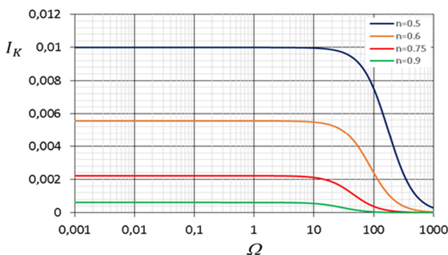
Figure 14. Dependency of the dispersion enhancement coefficient with dimensionless frequency and flow index for Re = 1 and \varepsilon = 0.1 .
