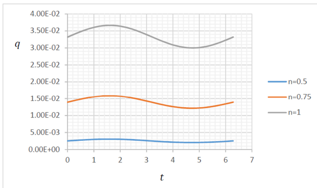
Figure 10. Discharge for \Omega = 1 , Re = 0.1 , \varepsilon = 1 .
