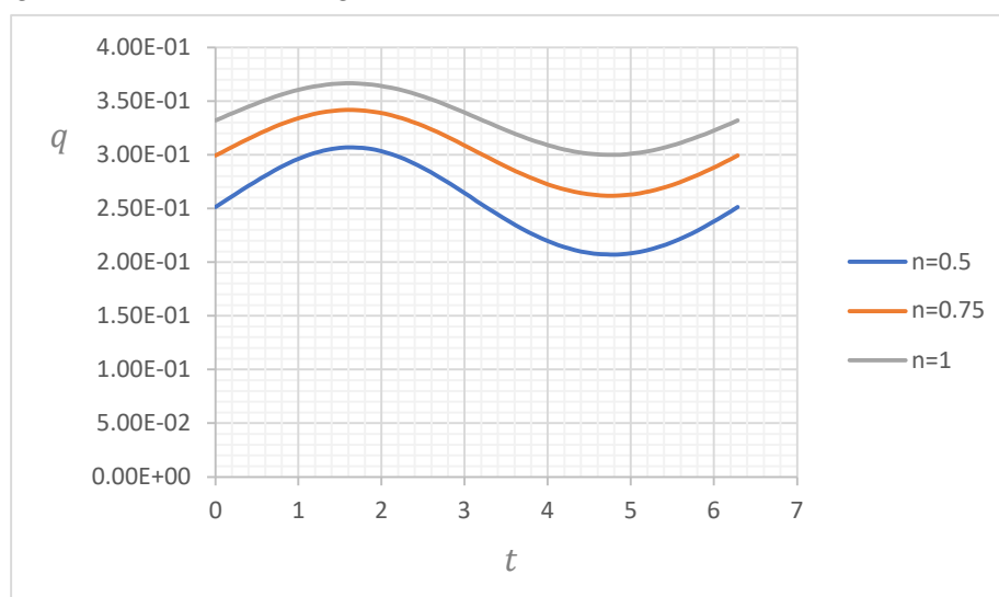
Figure 8. Discharge for \Omega = 0.1 , Re = 1 , and \varepsilon = 0.1 .
