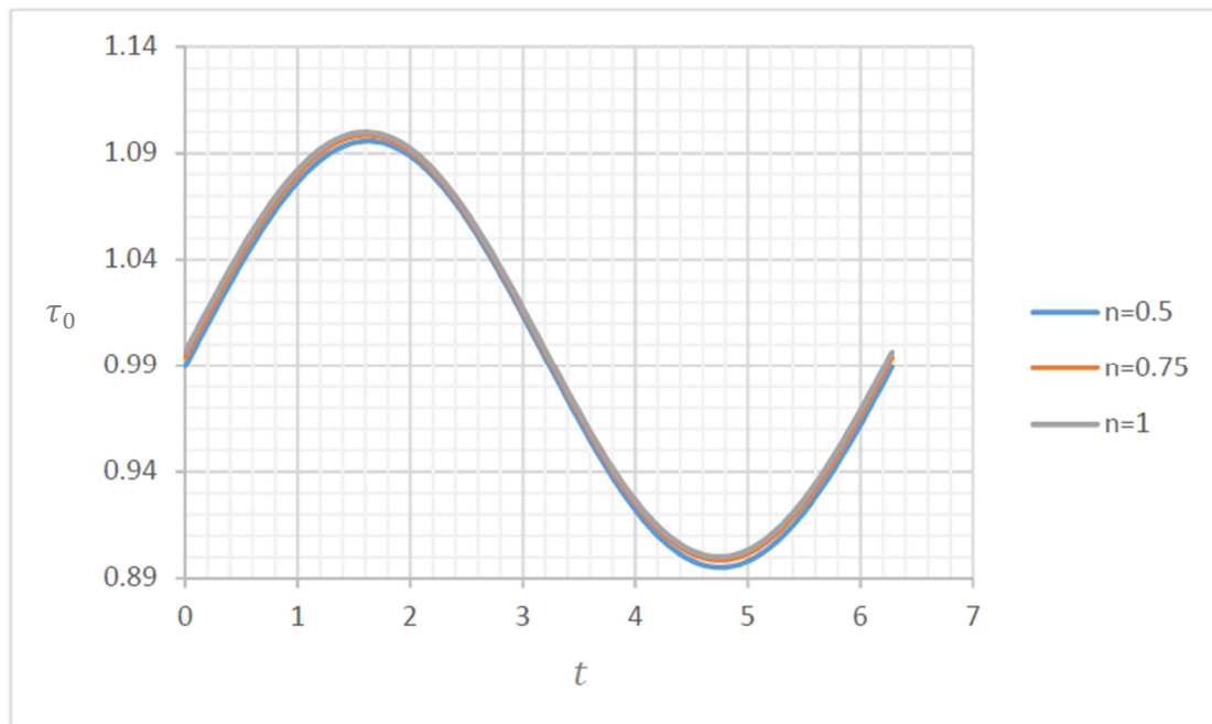
Figure 4. Wall shear stress for \Omega = 0.1 , Re = 1 , \varepsilon = 0.1 .
