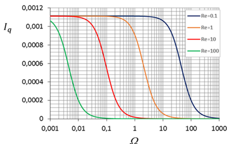
Figure 11. Dependency of the flow enhancement coefficient with dimensionless frequency and Reynolds number for n = 0.75 and \varepsilon = 0.1 .
