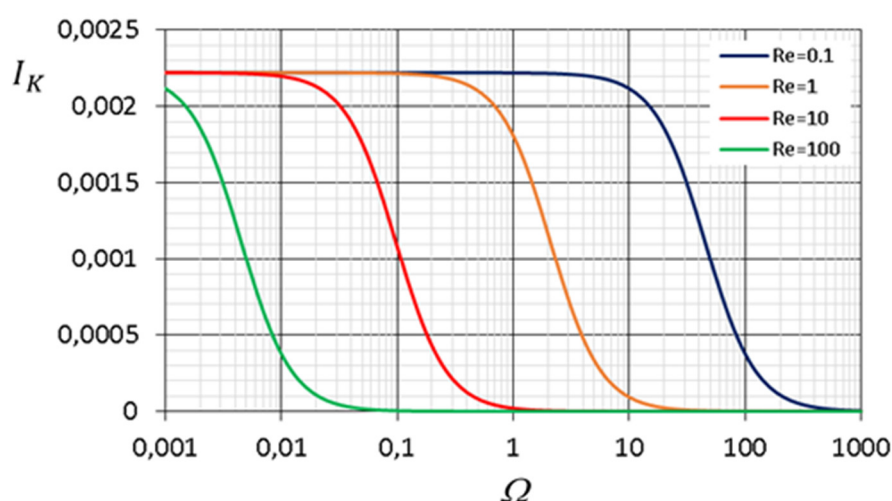
Figure 13. Dependency of the dispersion enhancement coefficient with dimensionless frequency and Reynolds numbers for n = 0.75 and \varepsilon = 0.1 .
