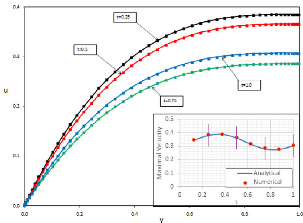
Figure 2. Comparison between analytical (lines) and numerical (symbols) velocity profiles. n = 0.5 , Re = 1 , \Omega = 1 , and \varepsilon = 0.1 . The inset shows the pulsation of the maximum velocity (reached at y = 1 ). The vertical lines in the inset are indicative of the times at which the velocity profiles were plotted in the main figure.
