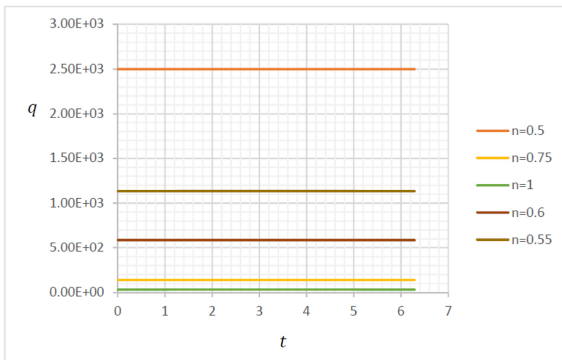
Figure 9. Discharge for \Omega = 1 , Re = 100 , \varepsilon = 0.1 .
