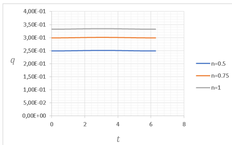
Figure 7. Discharge for \Omega = 100 , Re = 1 , and \varepsilon = 0.1 .
