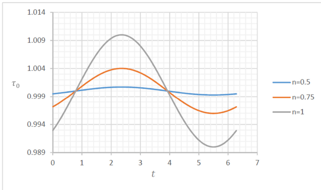
Figure 5. Wall shear stress for \Omega = 1 , Re = 100 , \varepsilon = 0.1 .
