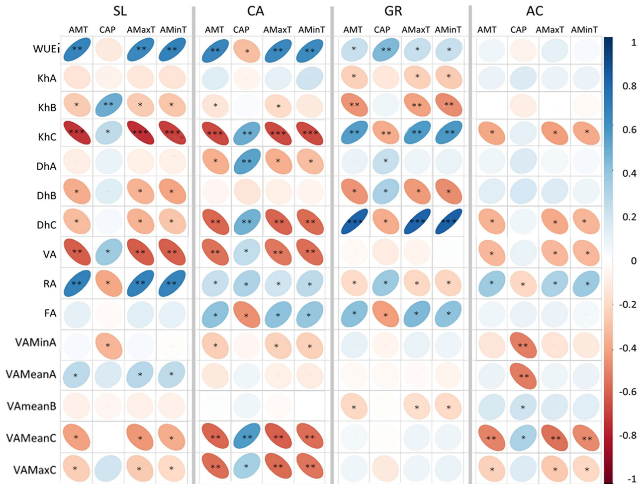
Fig. 4. Spearman's rank correlation coefficients among climatic variables and wood anatomical traits in the four vineyards: Santa Lucia (SL); Calvese (CA); Grottole (GR); Acquefredde (AC). Positive (blue) and negative (red) correlations ( r^2 ) are shown. *, **, ***, significant at P \leq 0.05 , 0.01 and 0.001 , respectively.
