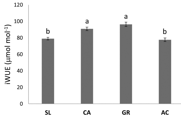
Fig. 3. iWUE values in trunk wood (rings corresponding to the years from 2015 to 2019) of grapevines from the four vineyards (x-axis): Santa Lucia (SL); Calvese (CA); Grottole (GR); Acquefredde (AC). Mean values and standard errors are shown. Different letters corresponded to significantly different values according to Duncan HSD test ( P \leq 0.001 ).
