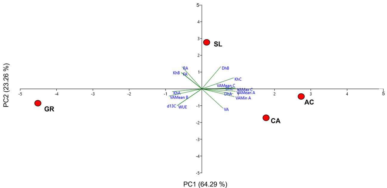
Fig. 5. Principal component analysis (PCA) biplot showing relationships between wood anatomical parameters and iWUE among the four vineyards (Santa Lucia, SL; Calvese, CA; Grottole, GR; Acquefredde, AC) during 2015–2019.
