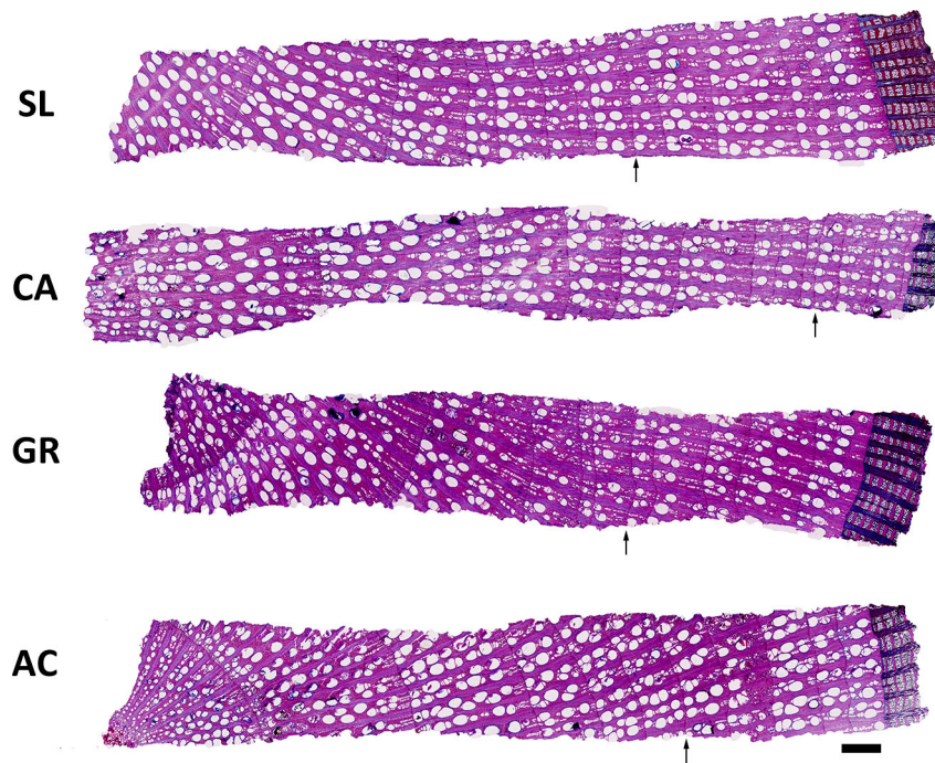
Fig. 1. Light microscopy views of cross sections of the trunk wood of grapevines from the four vineyards: Santa Lucia (SL); Calvese (CA); Grottole (GR); Acquefredde (AC). Images are at the same magnification. Arrows indicate the beginning of the 2015 ring. Scale bar = 500 \mu\text{m} .
