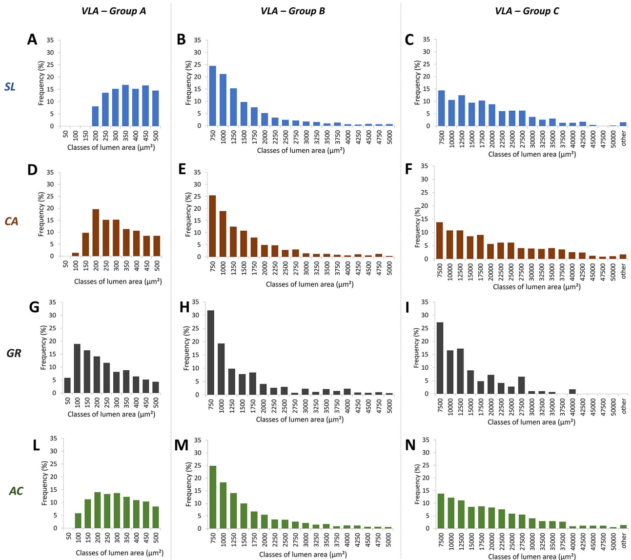
Fig. 2. Distribution of vessels in classes of lumen area in the three groups A (lumen area <500 \mu\text{m}^2 ), B (lumen area 500\text{--}5000 \mu\text{m}^2 ) and C (lumen area >5000 \mu\text{m}^2 ) in the trunk wood of grapevines from the four vineyards: A–C, Santa Lucia (SL); D–F, Calvese (CA); G–I, Grottole (GR); L–N, Acquefredde (AC).
