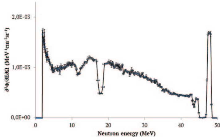
Fig. 1. – FLUKA neutron spectrum of 50 MeV protons lithium of 2 mm.
