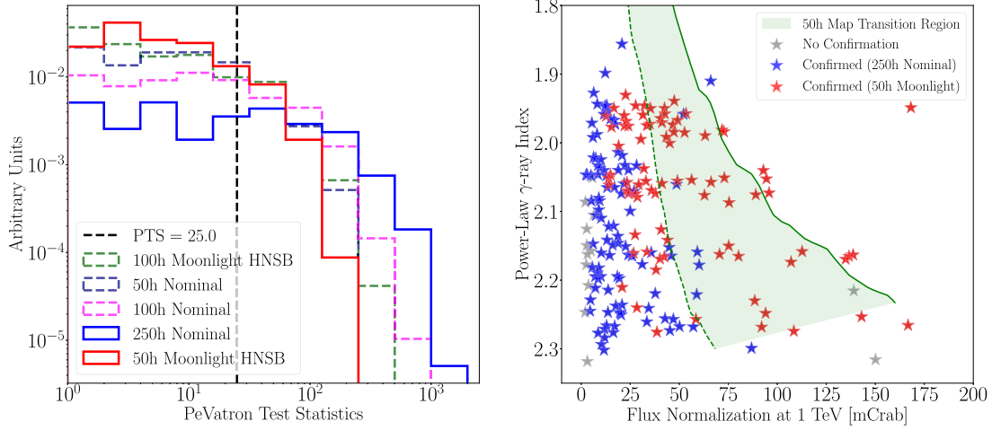
Fig. 10. The left panel shows the distribution of PTS values obtained from different observation strategies. The PTS identification threshold of 25 is used and shown as black dashed line. The right panel shows the spectral \gamma -ray parameters of simulated PeVatron SNRs as reconstructed from 10 h of CTA observations. Blue stars mark PeVatrons that can be confirmed after 250 h of follow-up observations. Red stars mark PeVatrons which can be confirmed with 50 h of moonlight observations. Grey stars indicate the PeVatron SNRs that cannot be confirmed with either follow-up observation strategies. The green area is the “transition region” for 50 h exposure shown in Fig. 4 (bottom left).
