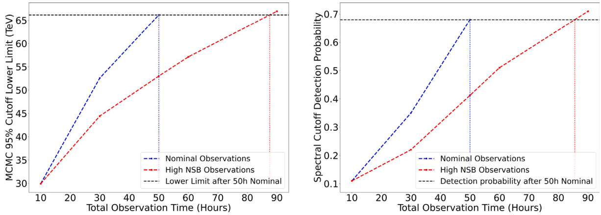
Fig. 11. Performance of SST subarray observations of HESS J1641–463 under moonlight conditions. Left Panel: 95% CL lower limit on the energy cutoff for sources without detection of a cutoff, i.e. TS_\lambda < 9 . To obtain the same limit as the 50 h nominal NSB follow up, the total observation time needed under moonlight conditions would be just under 90 h. Right Panel: Spectral cutoff detection probability as a function of total observation time. It is found that a detection probability of 68% obtained with 50 h nominal NSB can be achieved with just under 90 h high NSB, including 10 h from the GPS.
