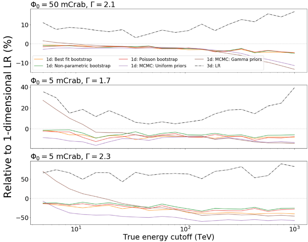
Fig. A.15. Point-like source energy cutoff sensitivity as a function of the true energy cutoff for different methods indicated by the legend in the upper panel relative to the respective sensitivity achievable with a 1-dimensional profile likelihood analysis. The different panels show the relative sensitivity for different point-like source parameters in terms of flux normalization \Phi_0 and index \Gamma , specified in the panel title. The instrument response functions of CTA south and 10 h of observation time at a zenith angle of 20^\circ are assumed.
