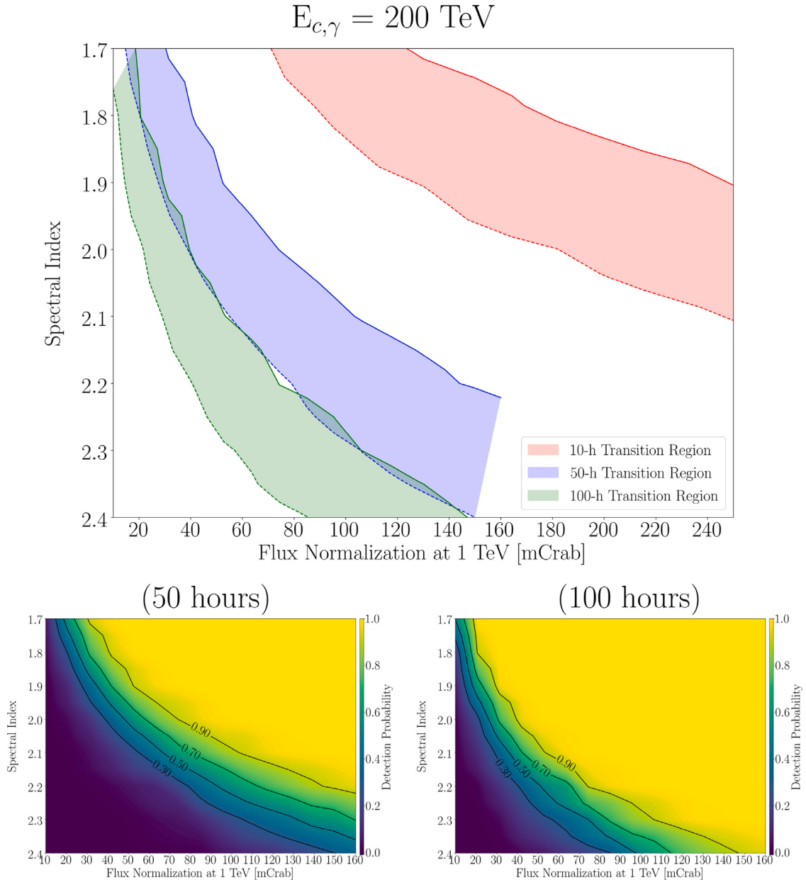
Fig. 5. Deep observation sensitivity of CTA to spectral cutoff features of point-like sources. As per Fig. 4, the top panel shows “transition region” for the detection of a spectral cutoff with true value of 200 TeV. The performance corresponding to 10 h, 50 h, and 100 h of CTA data is shown in red, blue and green. The corresponding spectral cutoff detection maps for 50 h and 100 h observations are given at the bottom left and right panels, respectively.
