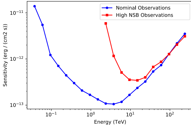
Fig. 9. Comparison of the CTA point-like source sensitivity for 10 h observation for different observations conditions. Nominal observations correspond to the CTA Omega array under conditions of astronomical darkness. High NSB observations correspond to the SST sub-array of CTA under conditions of 80% full moon illumination.
