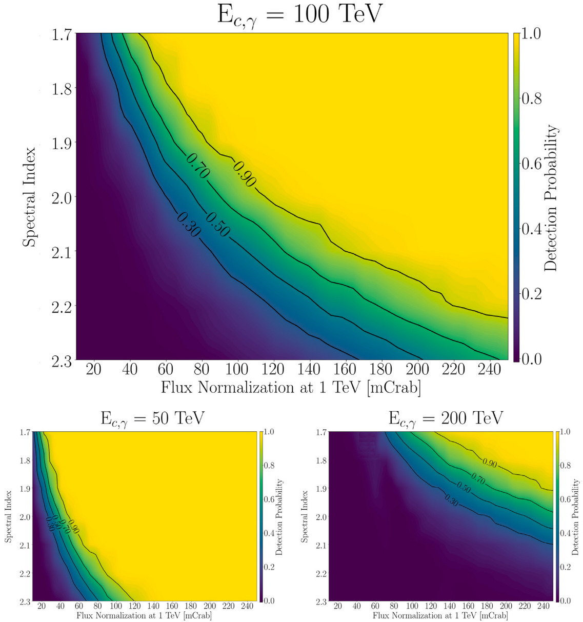
Fig. 1. Spectral cutoff detection probability maps for 10 h of CTA observations of point-like sources. The abscissa shows the true flux normalization, \phi_0 , at 1 TeV and the ordinate shows the true spectral index, \Gamma , of an ECPL model. The maps are generated for true cutoff energies of E_{c,\gamma} = 50 TeV (lower left panel), E_{c,\gamma} = 100 TeV (upper panel) and E_{c,\gamma} = 200 TeV (lower right panel). A TS_{\lambda} threshold of 25 is assumed. The colour code shows the \gamma -ray spectral cutoff detection probability, while the black lines are the cutoff detection probability contours at 0.3, 0.5, 0.7 and 0.9 levels. For comparison, 100 mCrab and 200 mCrab values correspond to differential flux level at 1 TeV of 3.84 \times 10^{-12} \text{ cm}^{-2} \text{ s}^{-1} \text{ TeV}^{-1} and 7.68 \times 10^{-12} \text{ cm}^{-2} \text{ s}^{-1} \text{ TeV}^{-1} , respectively.
