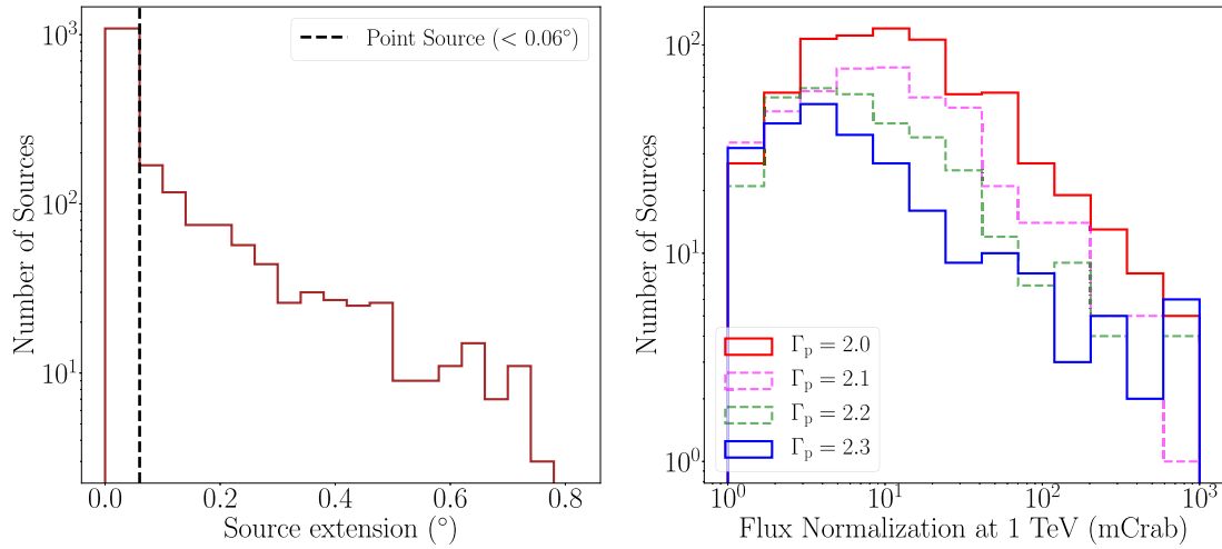
Fig. 6. Properties of detected SNRs from 200 simulated Galaxy samples. Left panel: Distribution of the angular extension of SNRs shown for all \Gamma_p values between 2.0 and 2.3. The vertical line marks the size up to which sources are detected as point-like by CTA at energies around 800 GeV. Right panel: Distributions of the true \gamma -ray flux normalization at 1 TeV, originating from true SNR proton spectral indices of \Gamma_p = 2.0 (solid red), \Gamma_p = 2.1 (dashed magenta), \Gamma_p = 2.2 (dashed green) and \Gamma_p = 2.3 (solid blue), are shown.
