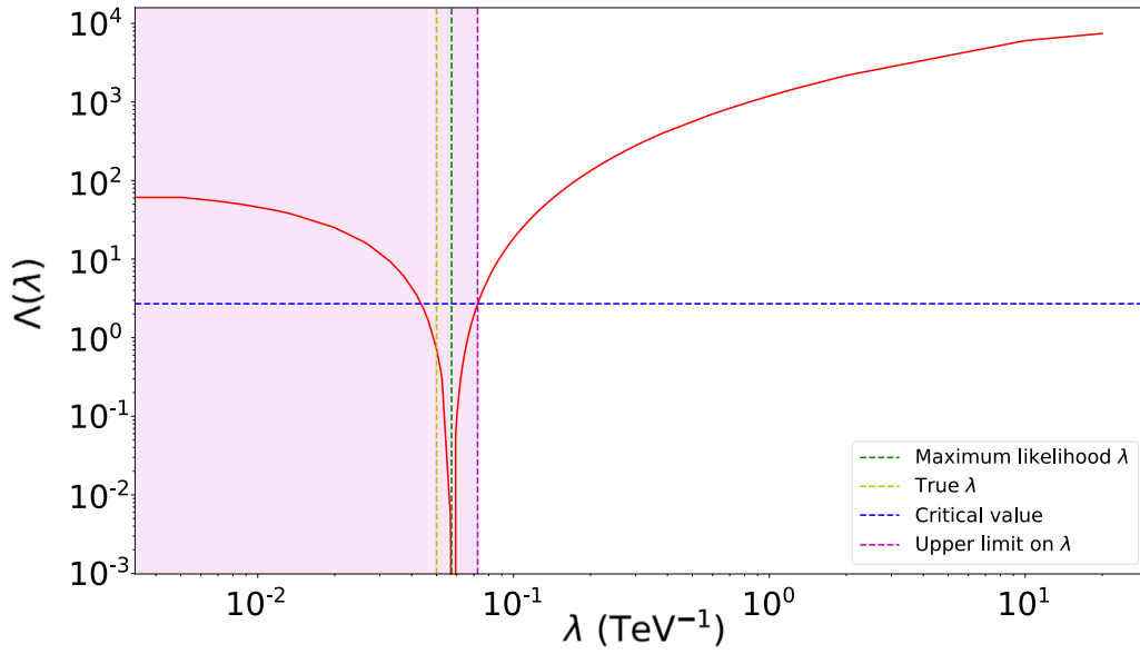
Fig. A.12. Shown in red is the likelihood ratio statistic \Lambda(\lambda) for the analysis of a typical \gamma -ray source with true exponential cutoff at 20 TeV. The maximum likelihood estimator \hat{\lambda} = \max(0, \lambda^{\text{ML}}) for non-negative \lambda is shown as green vertical line. The yellow line shows the true value of \lambda , i.e. \lambda^{\text{true}} = 1/20 \text{ TeV}^{-1} . The blue horizontal line indicates the critical value, \Lambda_{\text{crit}} \approx 2.71 , for a CL of CL = 0.95. The upper limit on \lambda is constructed at 95% CL as intersection of \Lambda(\lambda) with the horizontal critical value in the interval [\hat{\lambda}, \infty) , i.e. as upper end of the acceptance interval of the corresponding likelihood ratio test. The magenta coloured area indicates the range of inverse cutoff parameters which is not excluded at 95% CL.
