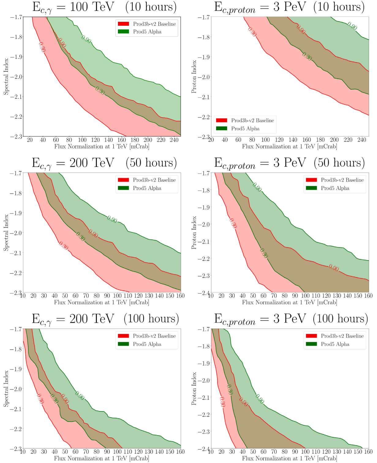
Fig. D.16. Comparison of “transition regions”, i.e. the regions between 30% and 90% detection probability, for the detection of a true spectral \gamma -ray cutoff (left panels) and the detection of a true PeVatron with a hadronic spectral cutoff at 3 PeV (right panels) after 10 (top), 50 (middle) and 100 (bottom) hours of observation. The “transition regions” shown as red and green shaded areas are obtained by using “Prod 3b-v2” (Baseline) and “Prod 5-v0.1” (Alpha) IRFs, respectively.
