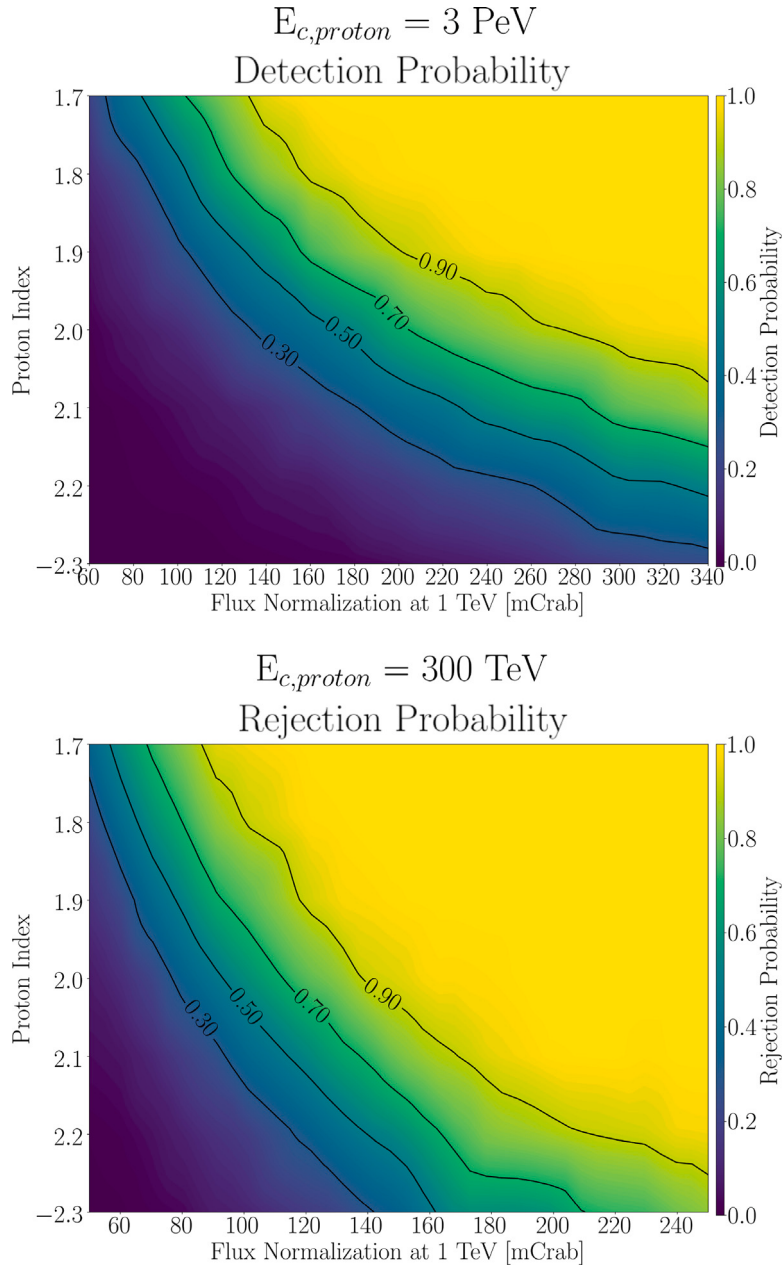
Fig. 3. PeVatron detection and rejection probability maps for 10 h of CTA observations of point-like sources. The abscissa shows the true observed \gamma -ray flux normalization at 1 TeV originating from pp interactions observed from Earth, while the ordinate shows true proton spectral index. The colour code shows the PeVatron detection (rejection) probabilities, while the black lines indicate the PeVatron detection (rejection) probability contours at 0.3, 0.5, 0.7, and 0.9 levels. Upper panel: PeVatron detection (PTS>25) probability map for a true proton energy cutoff at 3 PeV. Lower plot: PeVatron rejection (PTS<25) probability map for a true proton energy cutoff at 300 TeV. For comparison, 100 mCrab, 200 mCrab and 300 mCrab values correspond to differential flux level at 1 TeV of 3.84 \times 10^{-12} \text{ cm}^{-2} \text{ s}^{-1} \text{ TeV}^{-1} , 7.68 \times 10^{-12} \text{ cm}^{-2} \text{ s}^{-1} \text{ TeV}^{-1} and 1.15 \times 10^{-11} \text{ cm}^{-2} \text{ s}^{-1} \text{ TeV}^{-1} , respectively.
