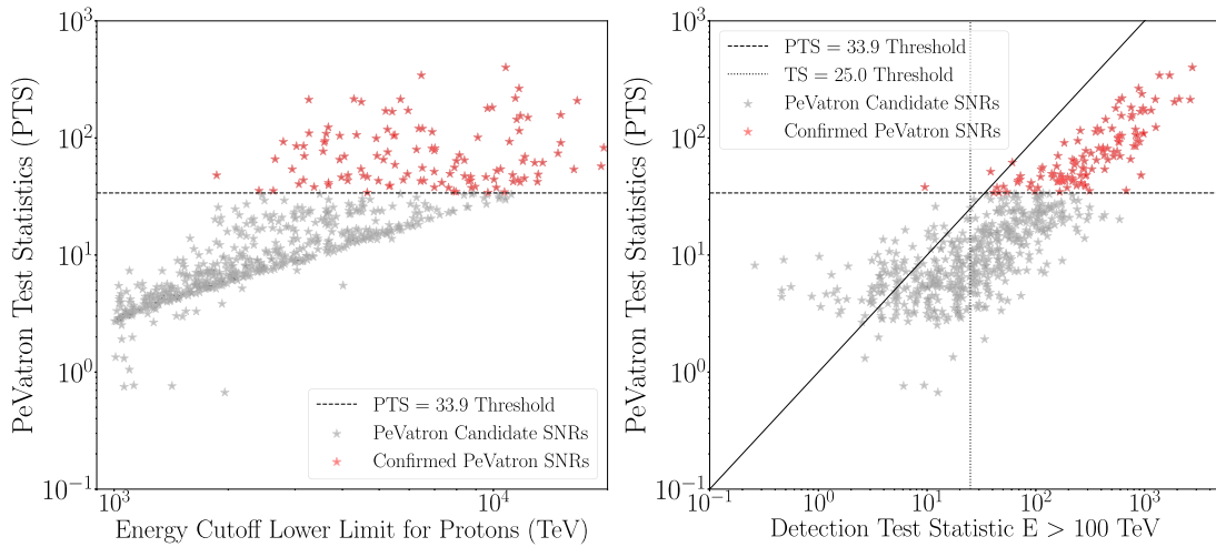
Fig. 8. Relation between the PTS and the lower 95% CL limit on the proton spectral cutoff (left) and detection test statistic, TS_{Det}^{100\text{ TeV}} , of the \gamma -ray flux above 100 TeV (right), combining all \Gamma_p values between 2.0 and 2.3. Confirmed PeVatrons are marked in red and PeVatron candidates are marked in grey. The PTS threshold of 33.9, corresponding to a global 5\sigma significance for 100 independent tests, is indicated with horizontal dashed black lines. In the right panel, the vertical line indicates the \gamma -ray detection threshold TS_{Det}^{100\text{ TeV}}=25 and the diagonal shows the equality PTS=TS_{Det} .
