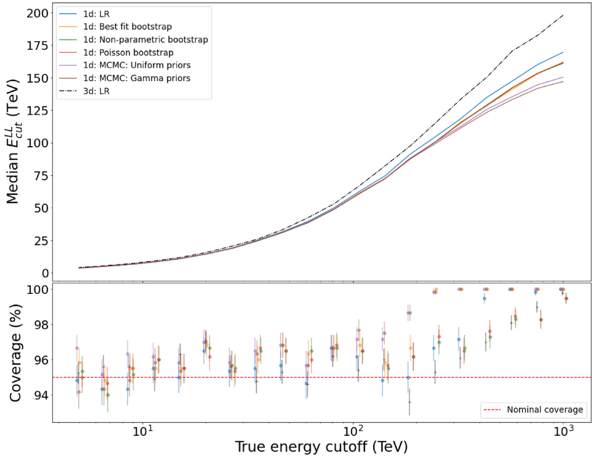
Fig. A.14. Comparison of different methods to derive a lower limit on the energy cutoff for a \gamma -ray point-like source with power-law index \Gamma = 2.1 and flux normalization \phi_0 = 50 mCrab. The instrument response functions of CTA South and 10 h of observation time at a zenith angle of 20^\circ are assumed. Upper panel: Median 95% CL lower limit on the energy cutoff as a function of the true energy cutoff. Colour codes for the different methods are indicated in the legend. Solid lines correspond to 1-dimensional analyses. Note that the green, orange and red solid lines overlap. The black dash-dotted line corresponds to profile likelihood limits derived with a 3-dimensional analysis. Lower panel: Coverage of the interval [E_{cut}^{LL}, \infty) for different methods to derive E_{cut}^{LL} = 1/\lambda^{\text{UL}} as a function of the true energy cutoff. The true energy cutoff is slightly shifted for each method to improve the visibility. Errorbars are approximate 68.3% CL intervals on the coverage, derived under the assumption of the normal approximation to the binomial distribution.
