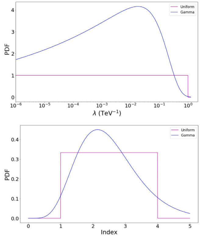
Fig. A.13. Investigated MCMC analysis prior distributions for the inverse energy cutoff \lambda (top) and power-law index \Gamma (bottom). Shown in magenta and blue are the assumed uniform and gamma distributed priors respectively. The uniform prior distributions for \lambda and \Gamma attribute a non-zero density within [0, 1] \text{ TeV}^{-1} and [1, 4] . The gamma prior distributions have shape (scale) parameters of 1.1 (0.182) and 7 (0.357), respectively for \lambda and \Gamma .
