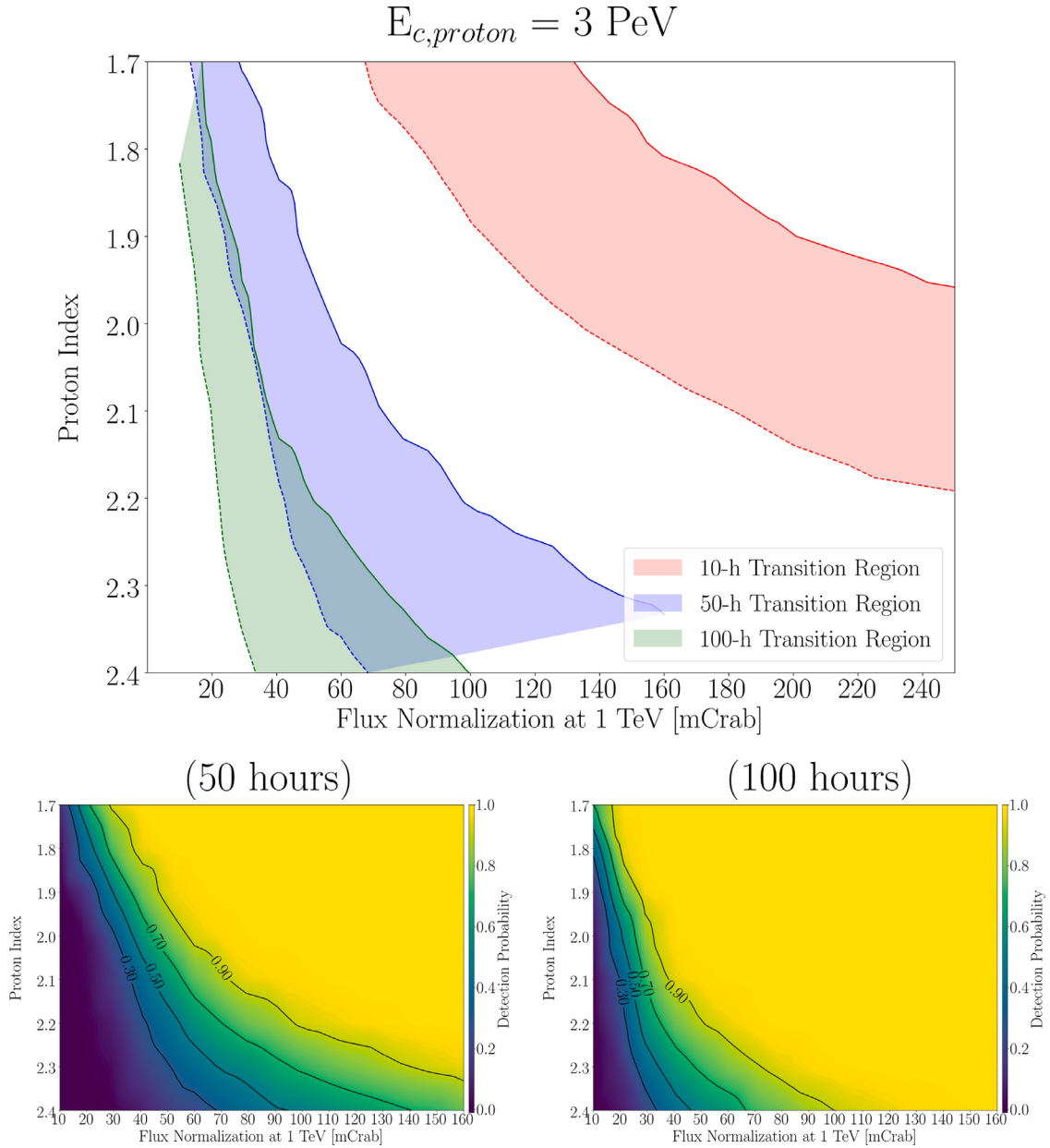
Fig. 4. Deep observation sensitivity of CTA to point-like PeVatrons. The top panel shows the comparison of the “transition regions”, i.e. the region between the detection probability contours of 30% (dashed lines) and 90% (solid lines), for a PeVatron with true proton cutoff at 3 PeV for 10 h, 50 h, and 100 h of CTA data. The corresponding PeVatron detection maps for 50 h and 100 h of observations with CTA are given at the bottom left and right panels, respectively.
