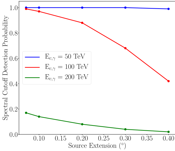
Fig. 2. Spectral cutoff detection probability as a function of the true source extension. The spectral cutoff detection probability is obtained from MC simulations of \gamma -ray ECPL spectral models with flux normalization \phi_0 (1 TeV) = 150 mCrab, spectral index \Gamma = 2.1 and cutoff energies E_{c,\gamma} = 50 TeV (blue), E_{c,\gamma} = 100 TeV (red) and E_{c,\gamma} = 200 TeV (green) for 10 h exposure.
