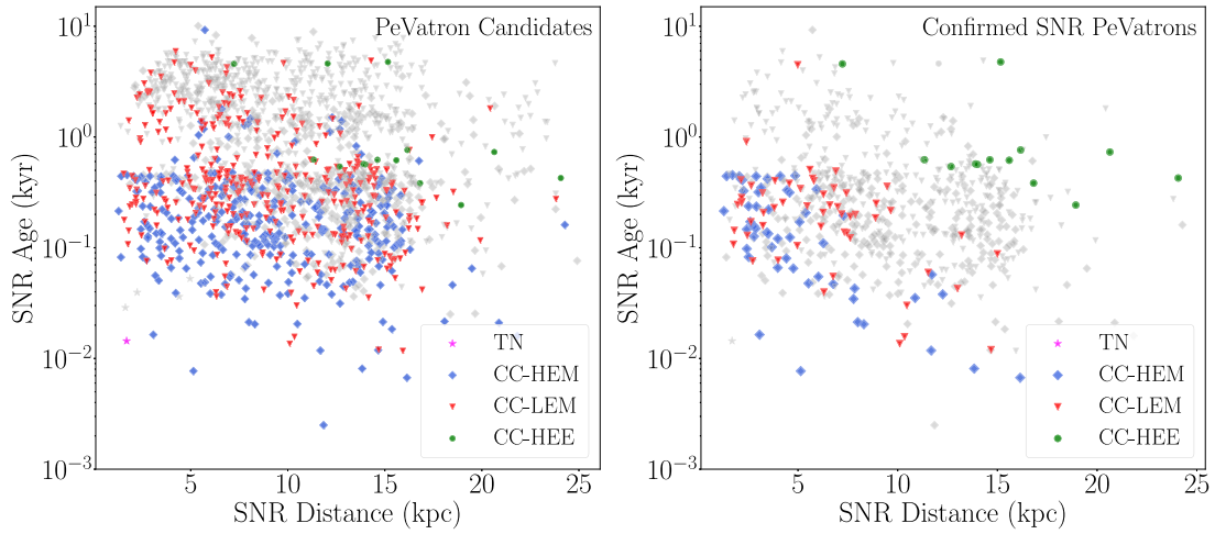
Fig. 7. Distance–age relation of SNRs from 200 Galaxy samples, combining all \Gamma_p values between 2.0 and 2.3. Left panel: Grey points mark all detected SNRs giving E_{c,p}^{LL} < 1 PeV, while PeVatron candidates ( E_{c,p}^{LL} > 1 PeV) with their corresponding SNR types are given in different colours. As detailed in the text, the gap around 600–700 years corresponds to the ‘transition age’ where the evolution of core-collapse SNRs evolves from dense wind to low density cavity. Right panel: Confirmed SNR PeVatrons (PTS > 33.9) and their progenitor types are given in different colours. Grey points mark, for comparison, all PeVatron candidates given with different colours in the left plot.
